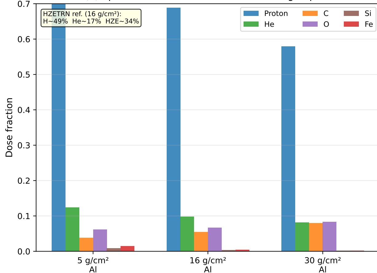
(b) Species dose breakdown at 3 shielding depths
