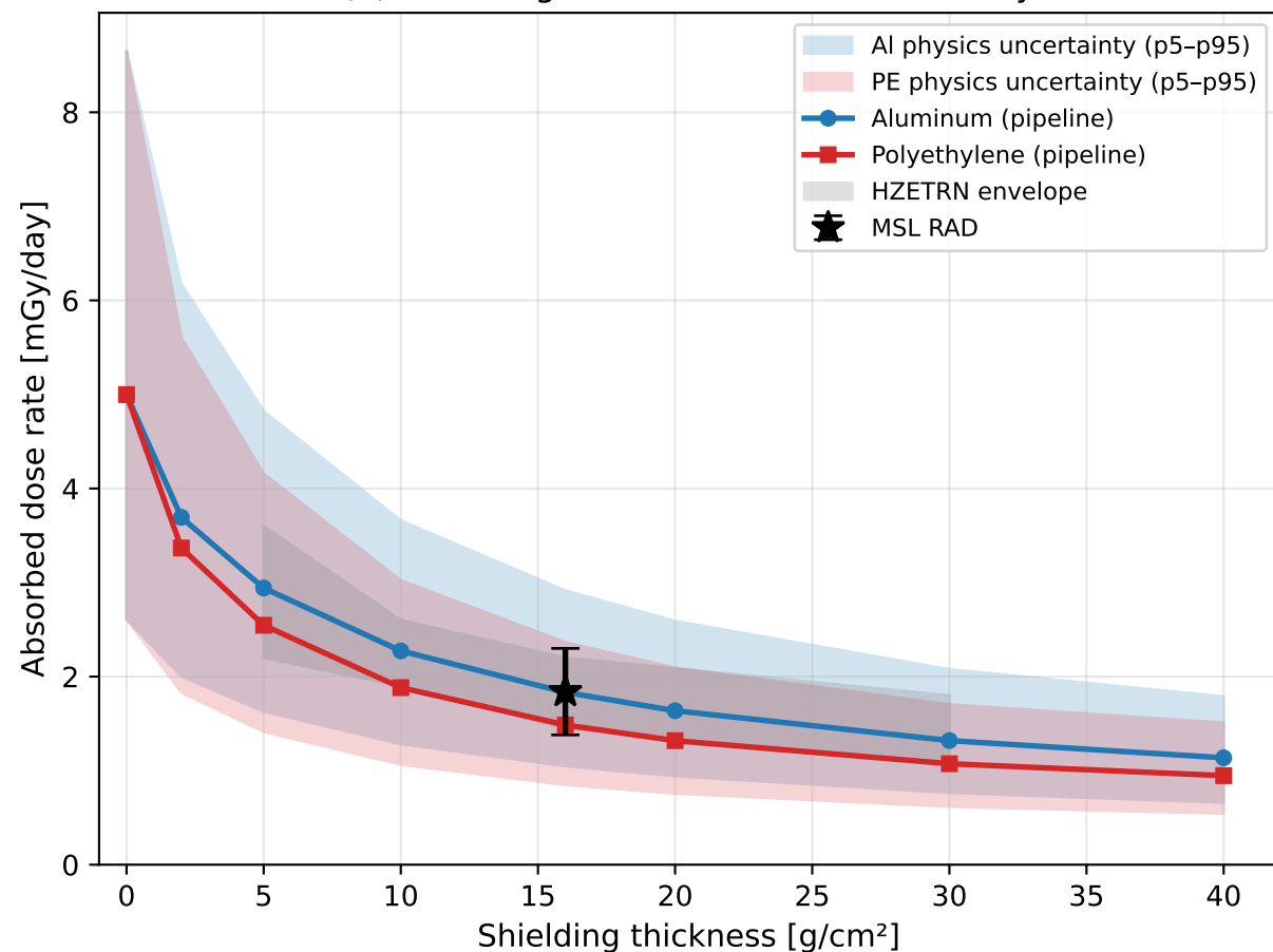
(a) Shielding effectiveness + uncertainty
