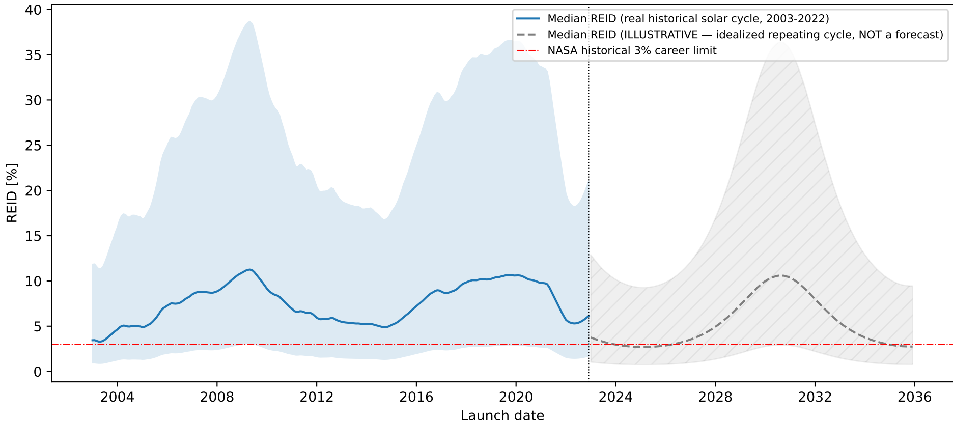
Mission cancer risk (REID) vs. launch date across the solar cycle (35-year-old male, 259-day transit, 16 g/cm 2 Al; shaded = p5-p95)
