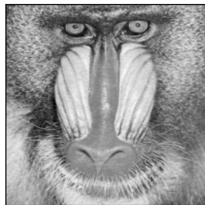
Watermarked (39.04 dB)
