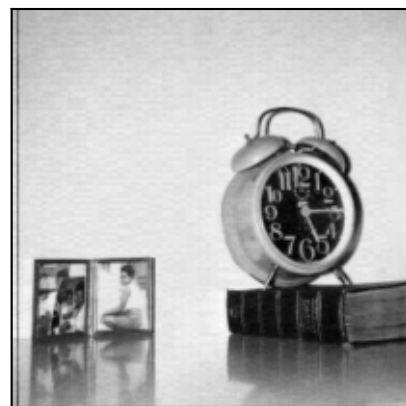
Watermarked (38.71 dB)
