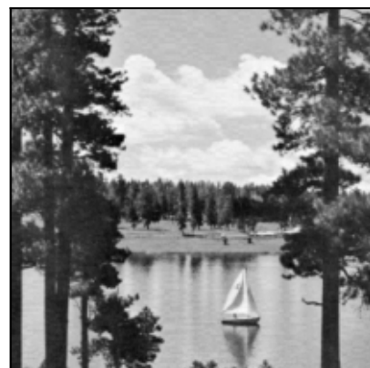
Watermarked (38.98 dB)
