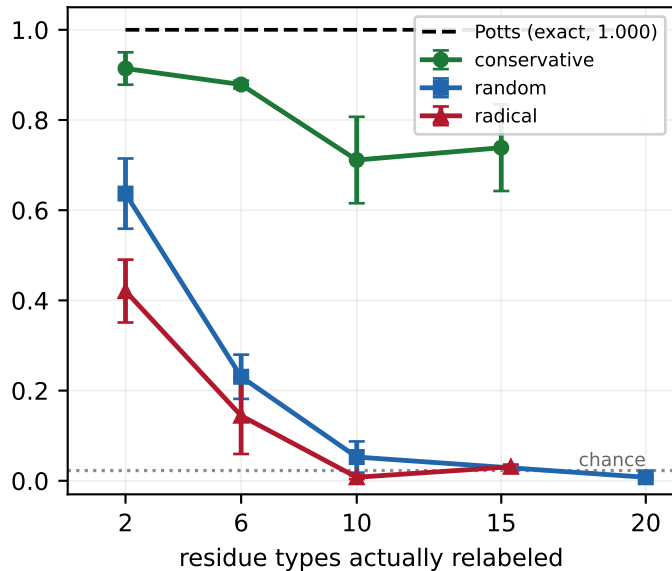
A ESM-2 650M (single sequence) 3 proteins
