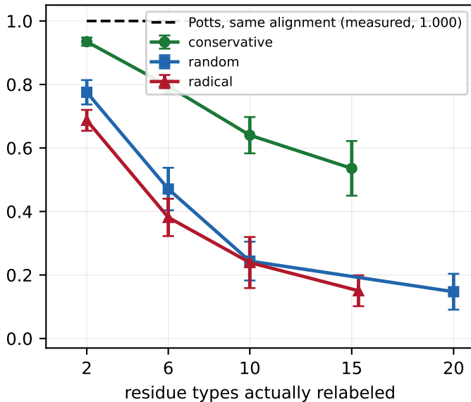
B MSA Transformer (reads the alignment) 4 families
