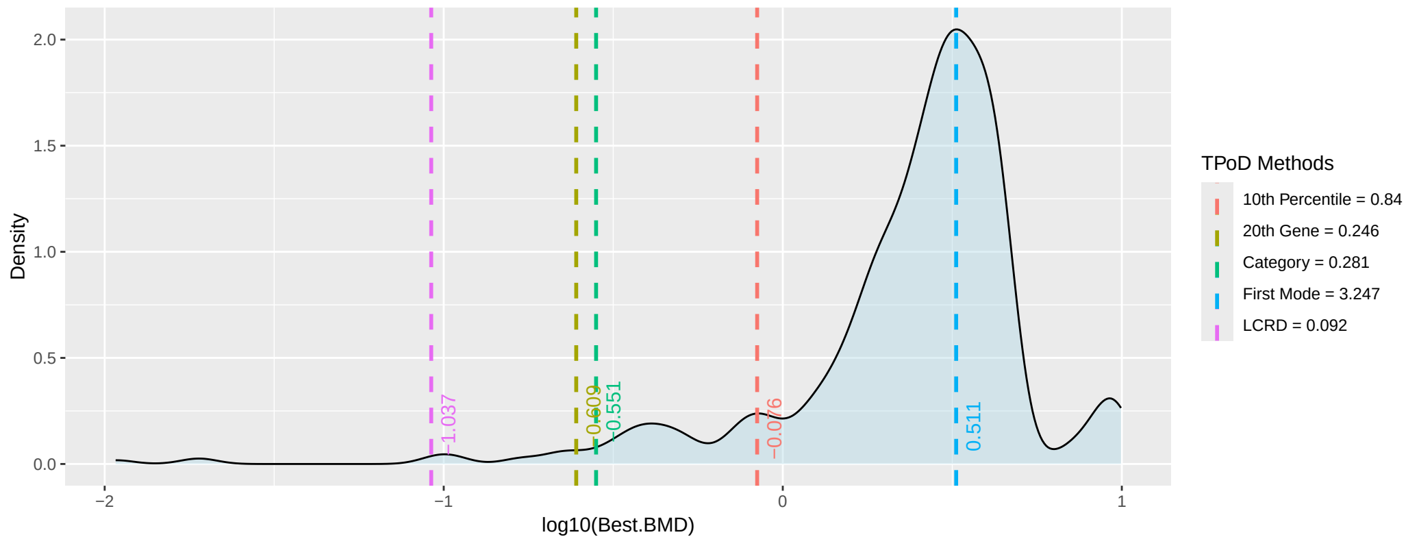
Distribution of Best BMD Values for BPC DRG = 860 | Top Dose = 10 | Low Dose = 0.001
