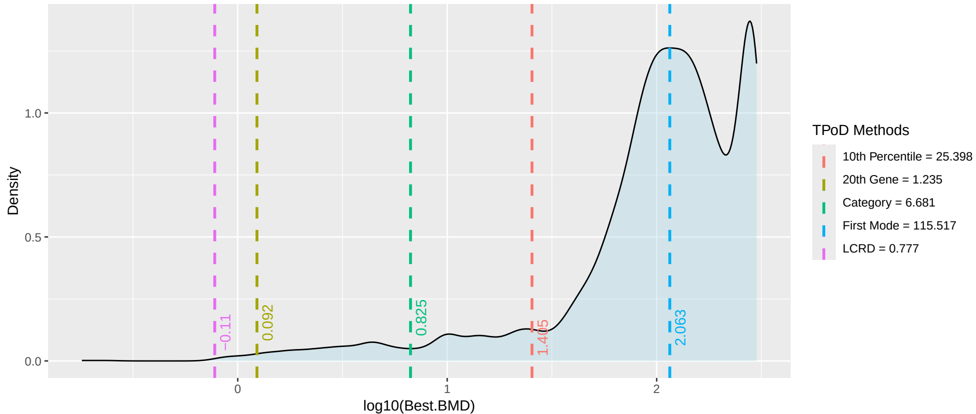
Distribution of Best BMD Values for MBHA
