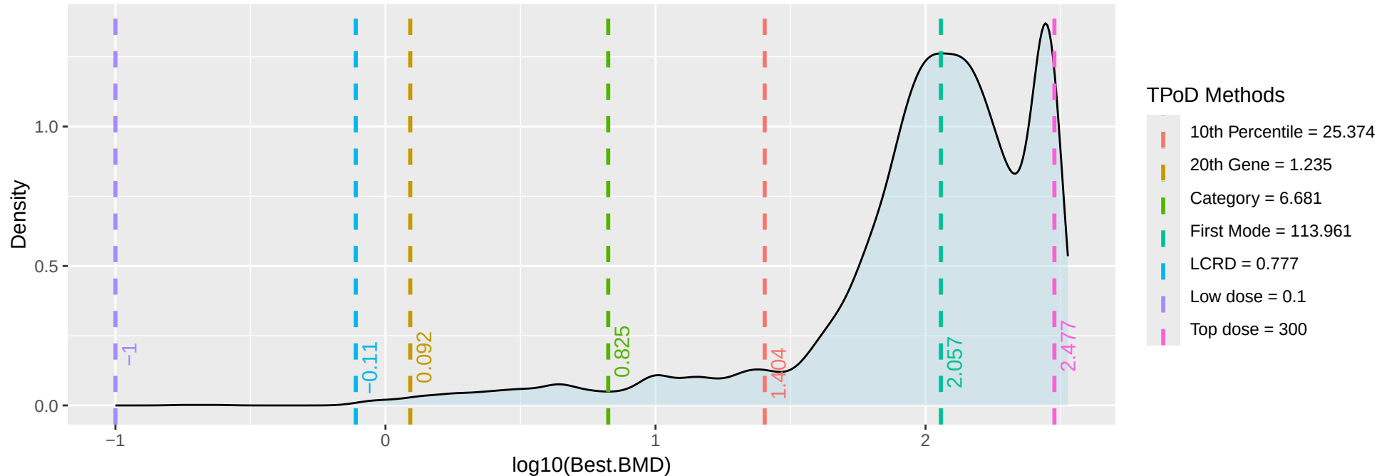
Distribution of Best BMD Values for MBHA DRG = 4578 | Top Dose = 300 | Low Dose = 0.1
