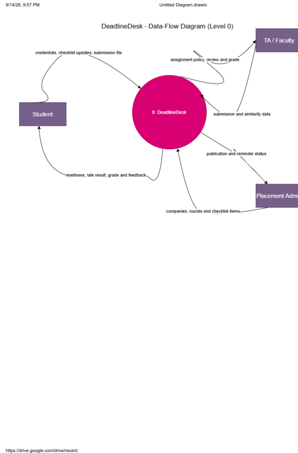
Figure 2: Level 0 data-flow diagram: external data exchanged with DeadlineDesk.
