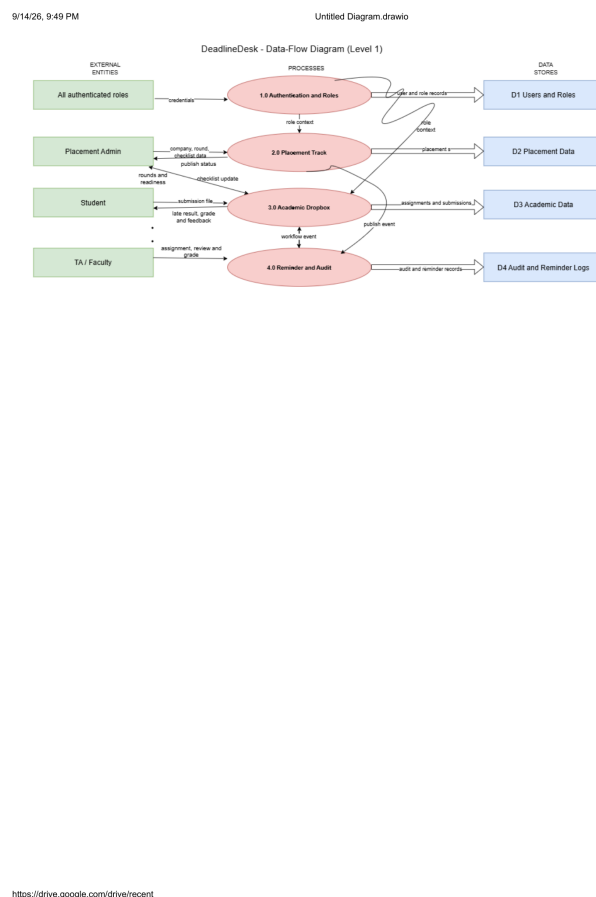
Figure 3: Level 1 data-flow diagram for implemented processes and persistent stores.
