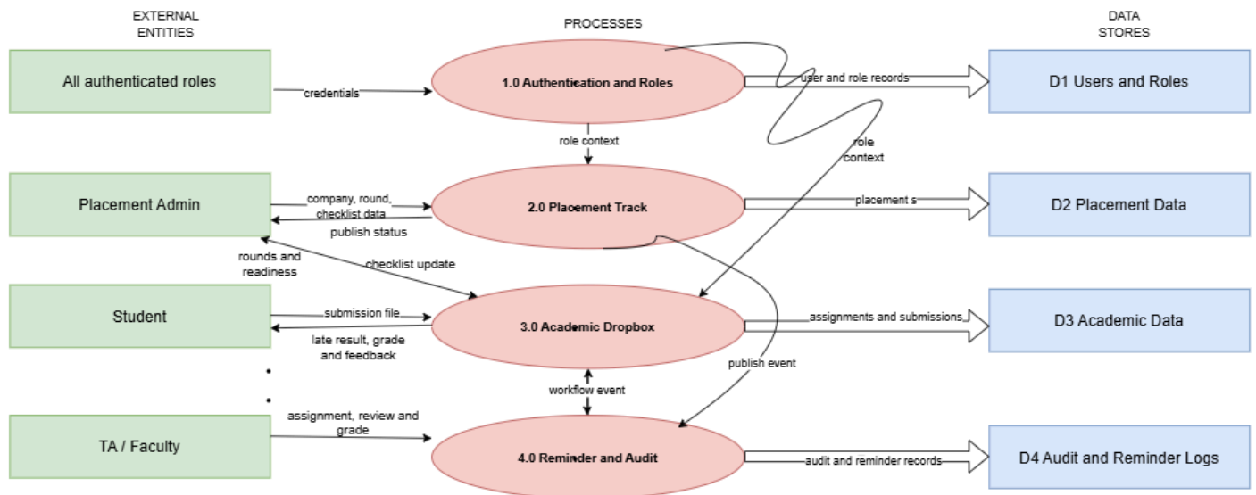
DeadlineDesk - Data-Flow Diagram (Level 1)
