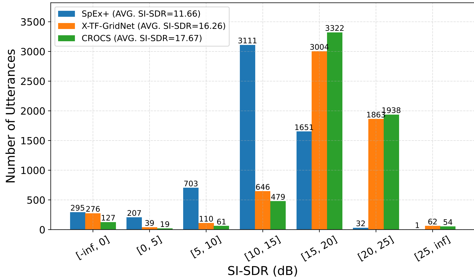
SI-SDR distribution
