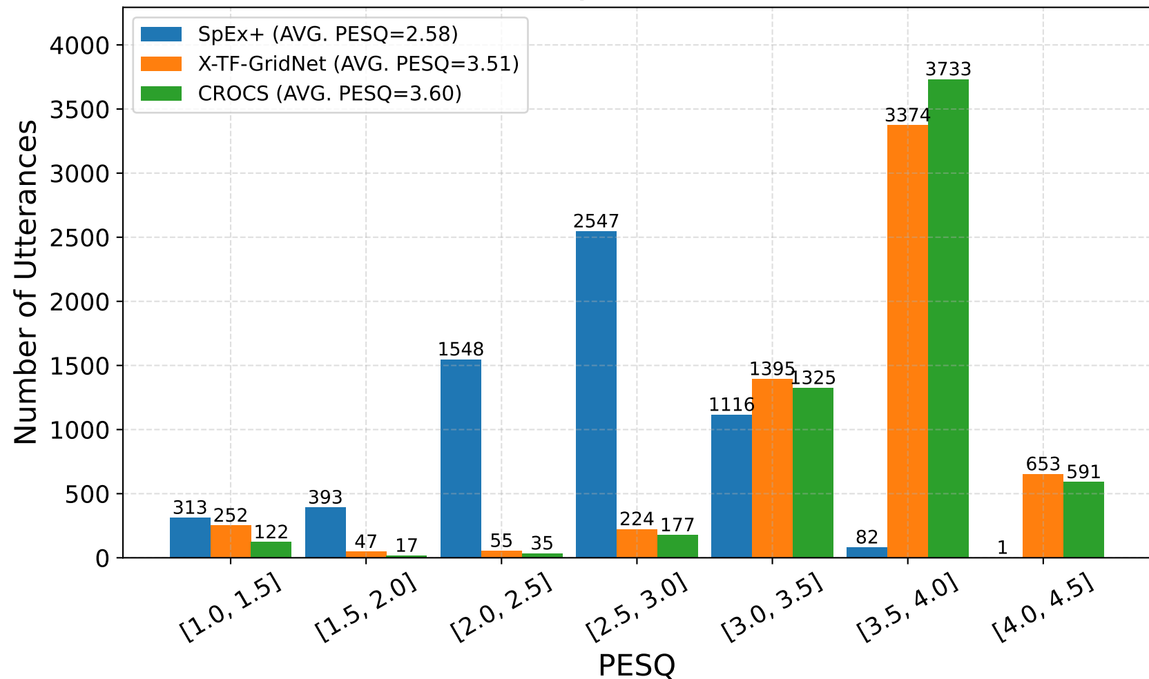
PESQ distribution
