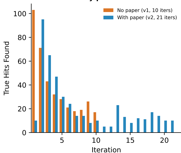
C Hit Discovery per Iteration
