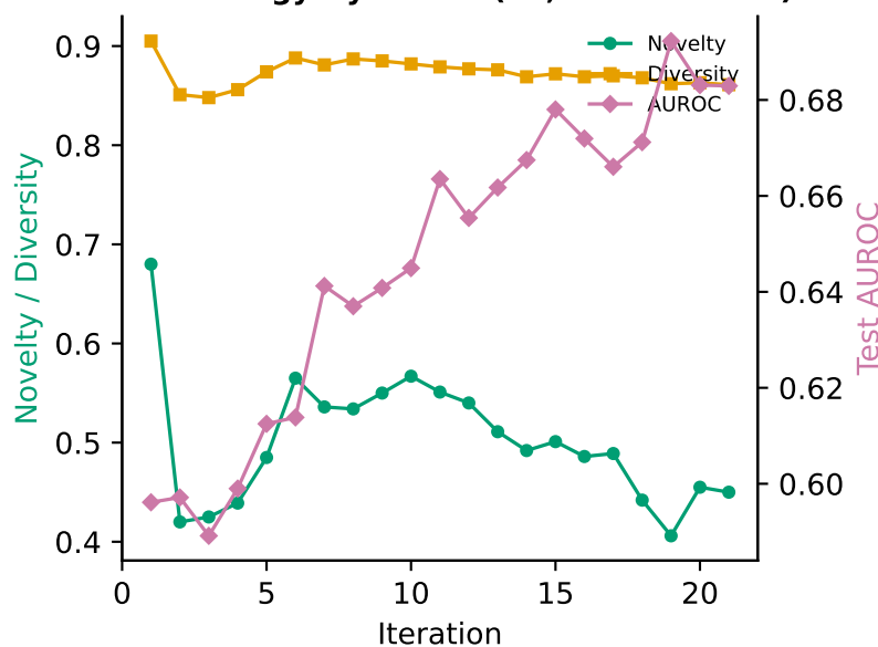
D Strategy Dynamics (v2, 21 iterations)
