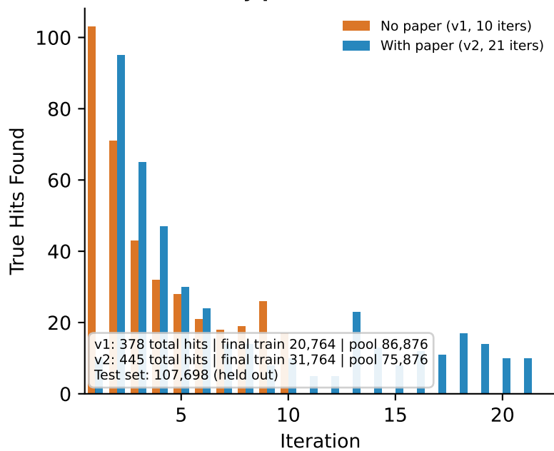
C Hit Discovery per Iteration
