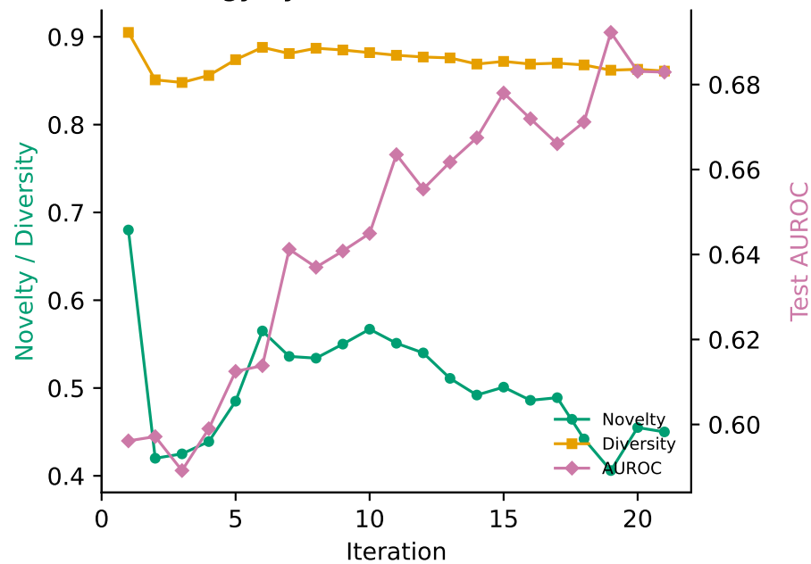
D Strategy Dynamics (v2)
