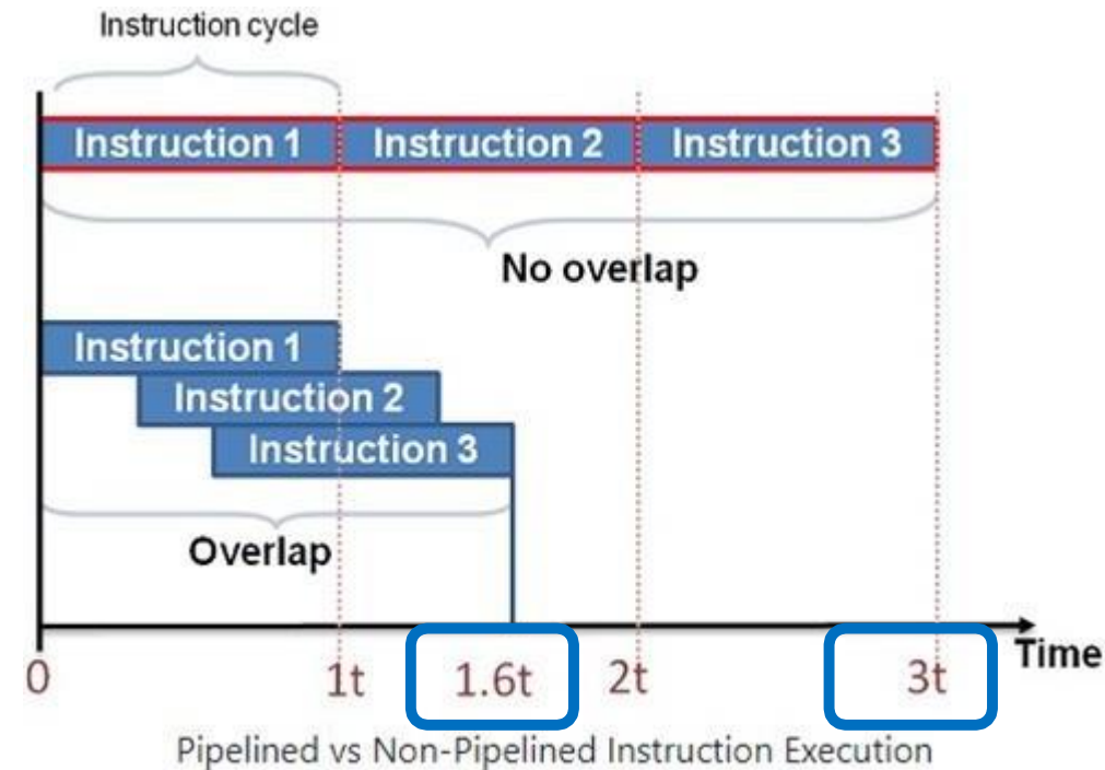
Pipelined Execution
