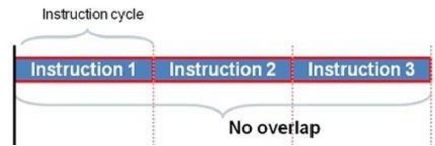
Non-pipelined Execution
