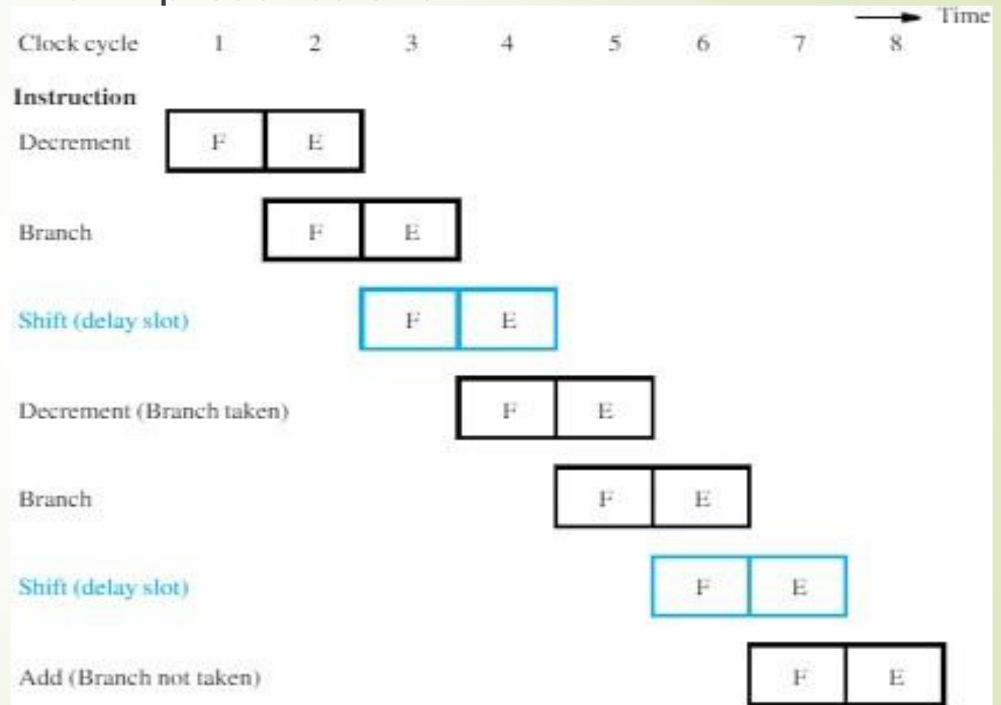
Figure 8.13 Execution timing showing the delay slot being filled during the last two passes through the loop in Figure 8.12b.
