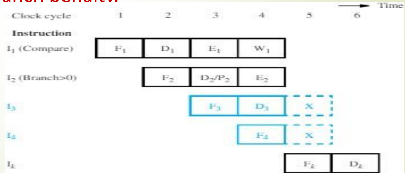
Figure 8.14 Timing when a branch decision has been incorrectly predicted as not taken.
