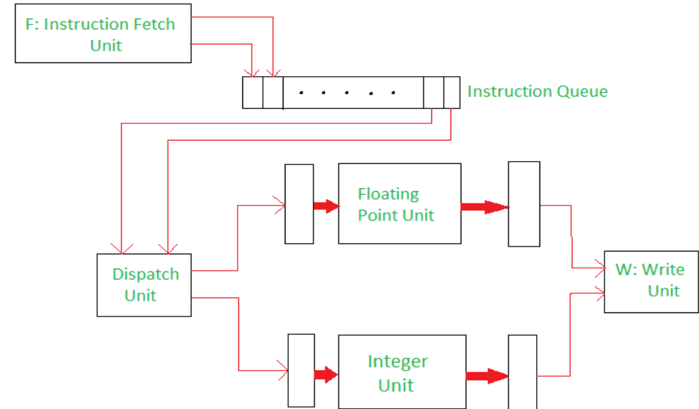
Processor with Two Execution Units
