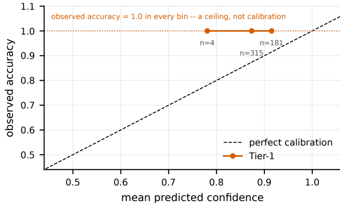
Tier-1 (TF-IDF), ECE = 0.1122
