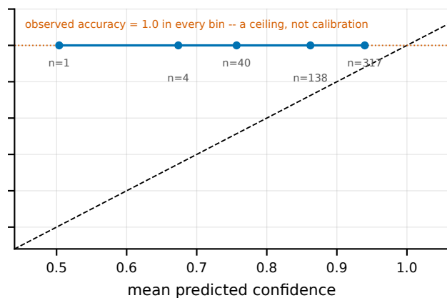
Tier-2 (BGE), ECE = 0.0992
