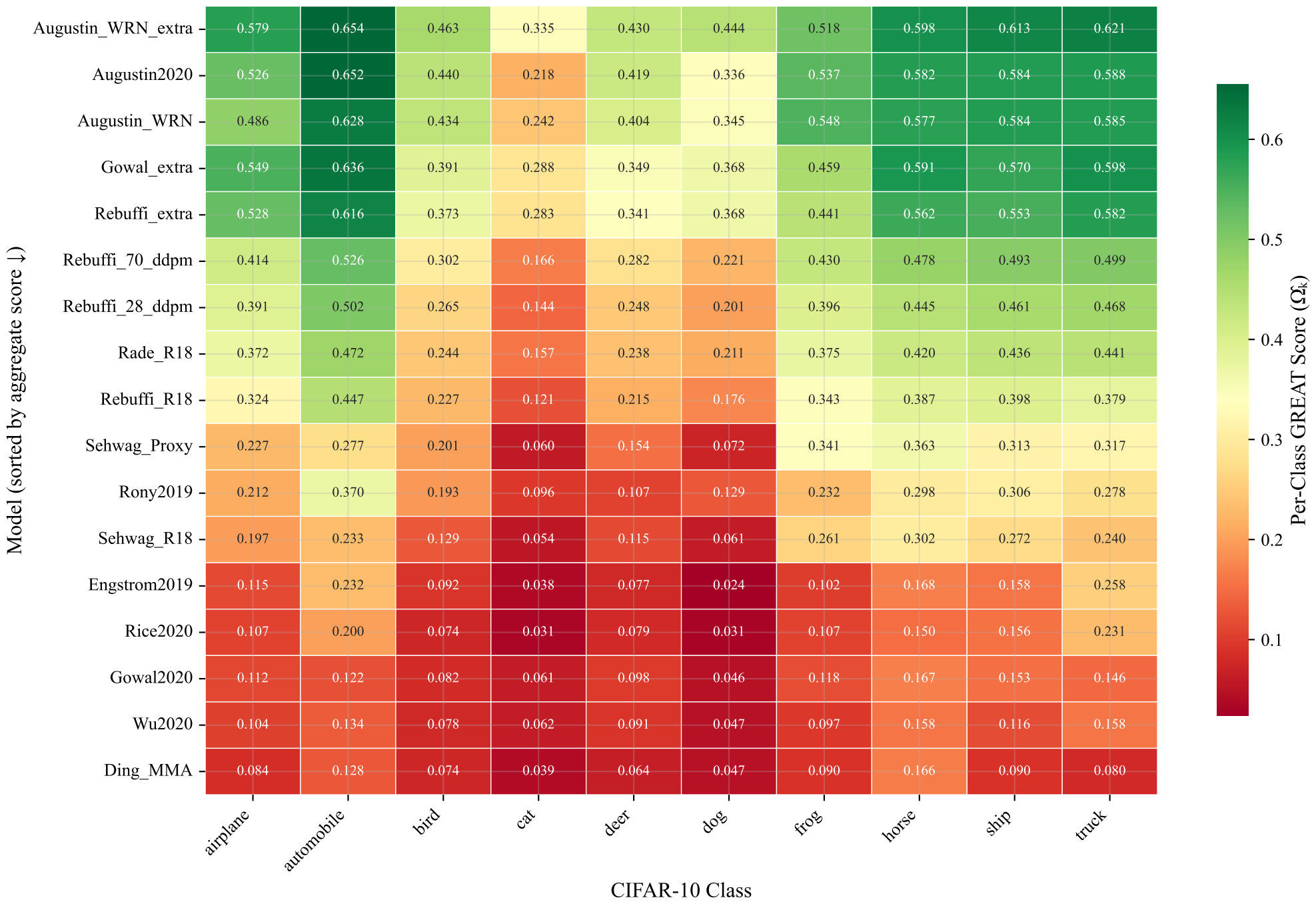
Class-Conditional Robustness Heatmap
