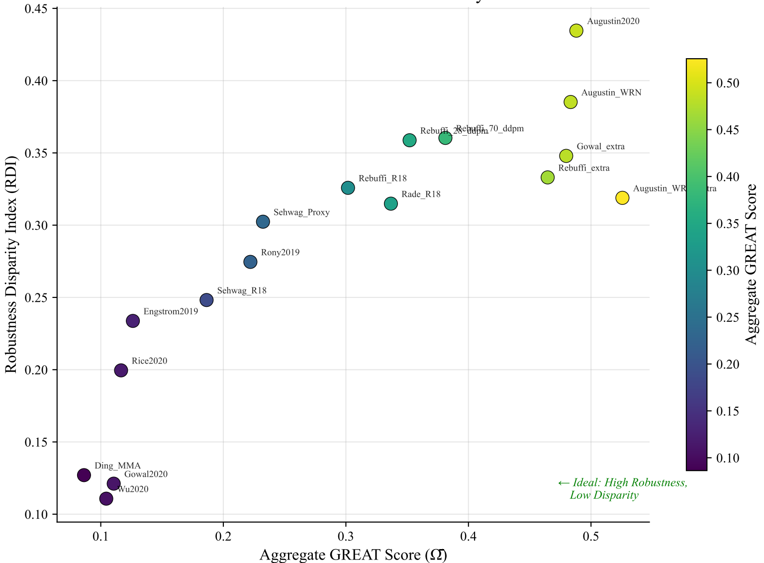
Robustness vs. Fairness: Pareto Analysis
