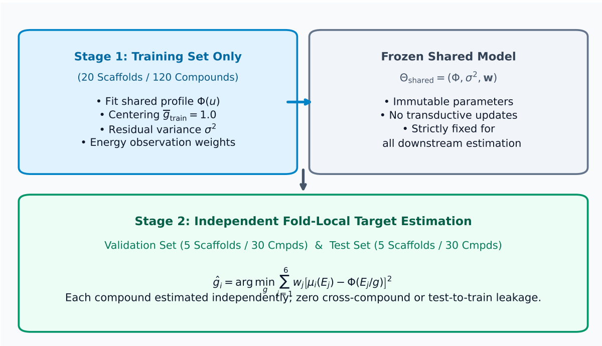
FIGURE 1: MURU Computational Architecture and Governance Boundary
