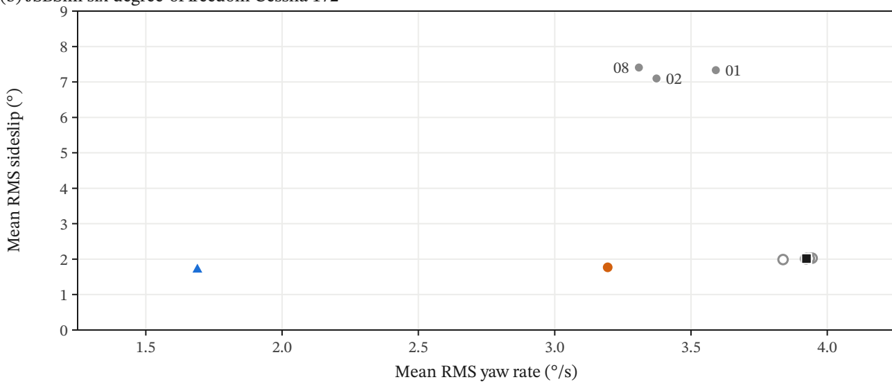
(b) JSBSim six-degree-of-freedom Cessna 172
