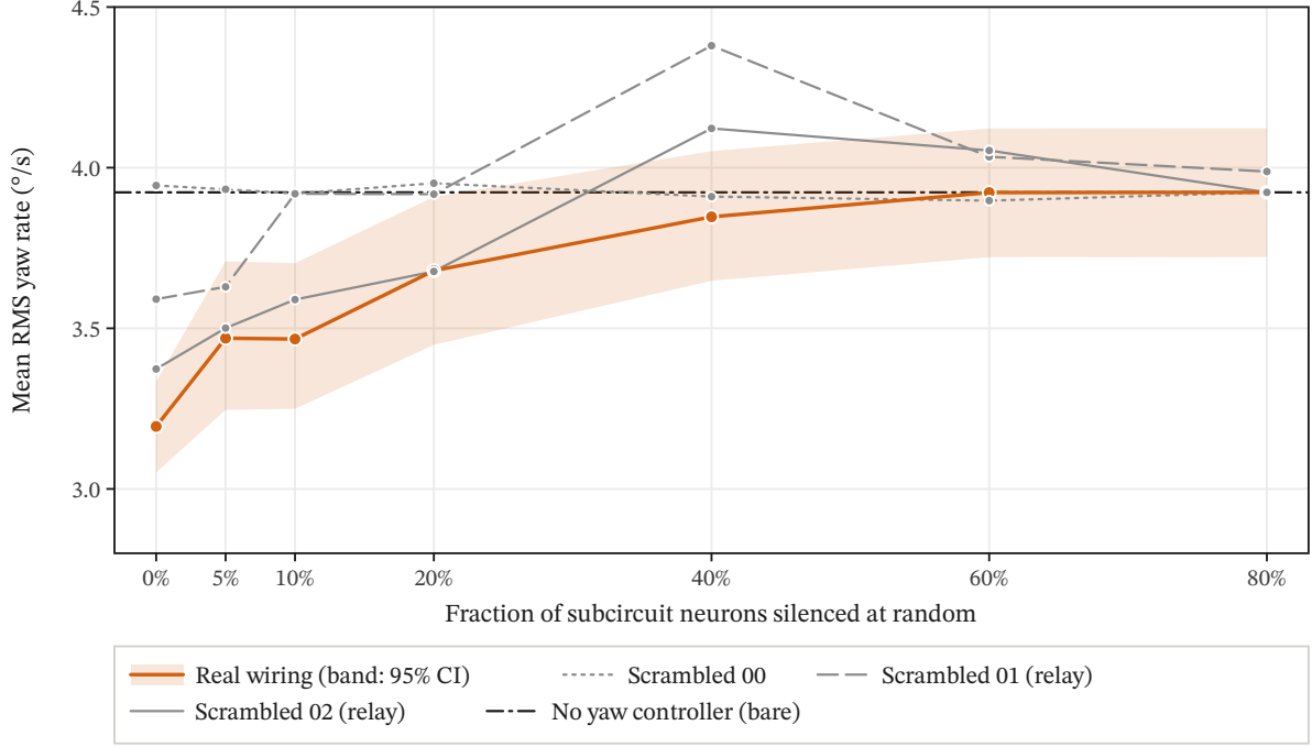
Figure 5. Mean RMS yaw rate against the fraction of neurons silenced at random. Mean over 20 test seeds (nested sets, the same neurons in every wiring), on the six-degree-of-freedom model. Each wiring keeps its tuned gain. The shaded band is the 95% bootstrap interval for the real wiring; the dash-dotted line is the bare airframe. The yaw damper, for reference, flies at 1.69 °/s. Bare: no yaw controller; on the six-degree-of-freedom model the wings-level roll hold common to every controller stays on.
