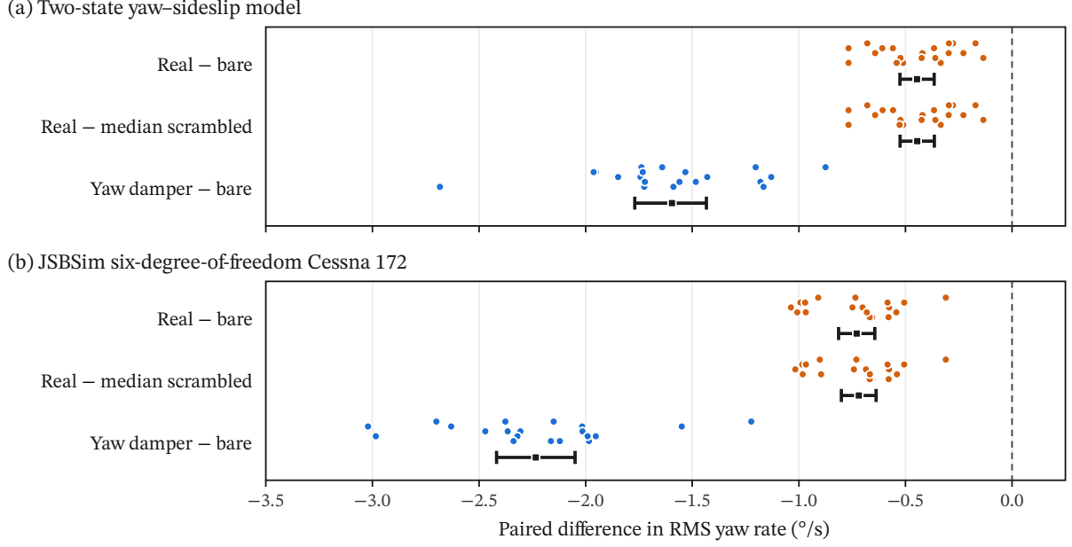
Figure 2. Paired differences in RMS yaw rate on the 20 held-out test seeds. Small dots: one per seed. Squares and bars: mean and 95% percentile bootstrap interval. Negative values favour the first-named controller. The real wiring helps on every seed; the yaw damper helps much more.
