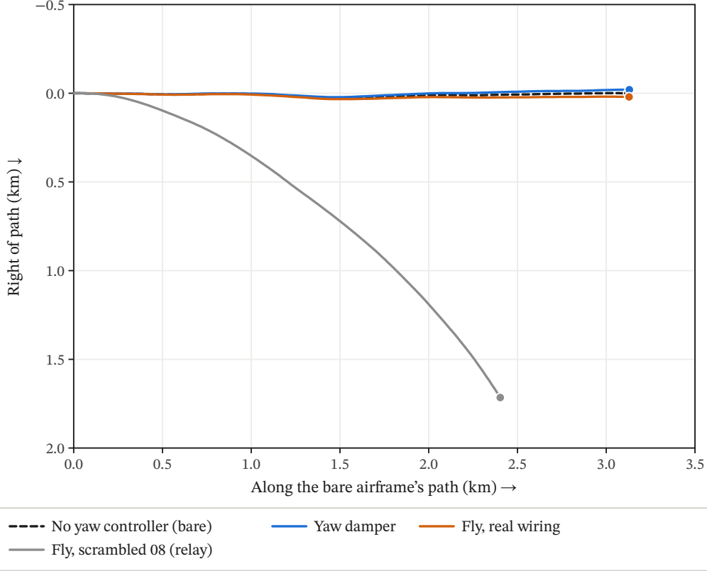
Figure 4. Ground tracks of the six-degree-of-freedom flights on test seed 100. Same turbulence random seed for all. JSBSim’s gust filter depends on each aircraft’s airspeed, so the gust histories differ slightly: at most about 0.06 m/s for the controllers shown, 0.47 m/s for the skidding relay. Plan view from above. Scrambled wiring 08 had the lowest training RMS yaw rate of the ten scrambled wirings, but it flies as a relay: the rudder sits at its stop, the aircraft skids in a steady right turn and ends 1.72 km off course (Section 3.3). The frame is aligned with the bare airframe’s start-to-end path, which runs left to right, so a turn to the right appears as a track bending downward; both axes have the same scale. Dots mark the end of each 60 s flight. Bare: no yaw controller; on the six-degree-of-freedom model the wings-level roll hold common to every controller stays on.
