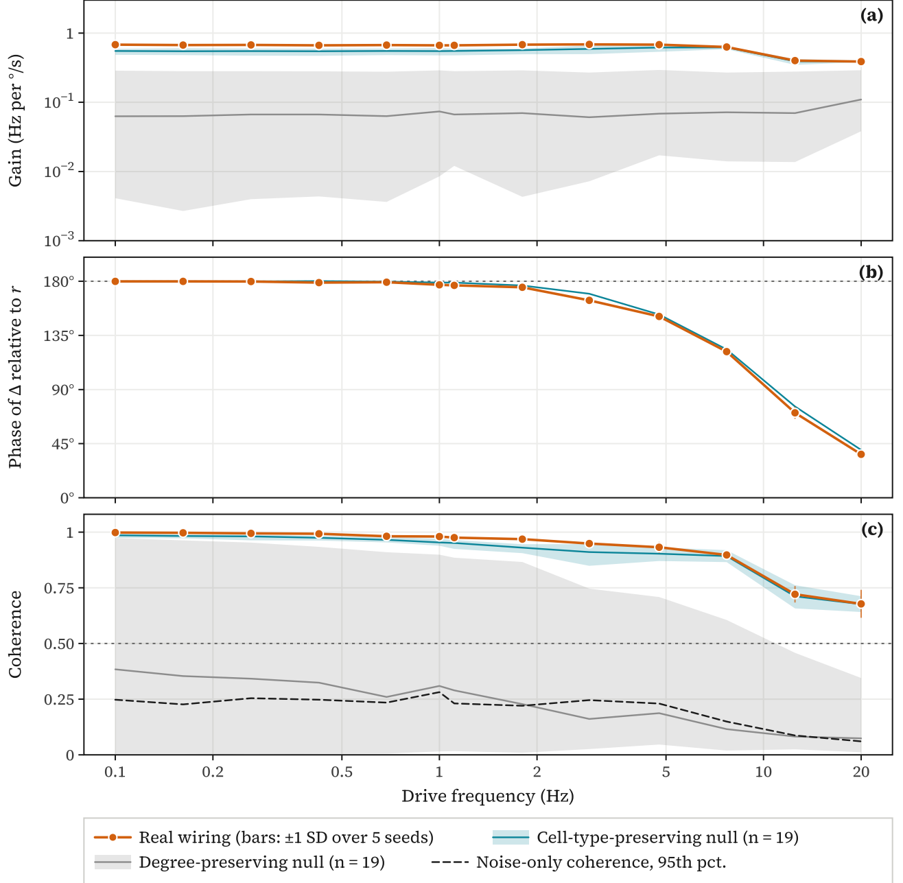
Figure 1. Open-loop frequency response of the real wiring and of both null models. Right-minus-left DNa02 rate \Delta in response to yaw rate r (100 °/s stepped sines, mean of 5 seeds). (a) Gain, (b) phase of \Delta relative to r (180° opposes the rotation), (c) coherence. Vertical bars on the real wiring: \pm 1 SD over the 5 seeds. In (a) and (c), bands span the minimum to maximum of the 19 rewirings of each null and thin lines are their medians. Panel (b) shows the cell-type-preserving median only (no band), because most degree-preserving rewirings have too little coherence for a phase to be defined; its dotted line marks 180°. The dotted line in (c) is the H1 threshold; the dashed line is the 95th percentile of the coherence of a sine against white noise, computed for a single seed.
