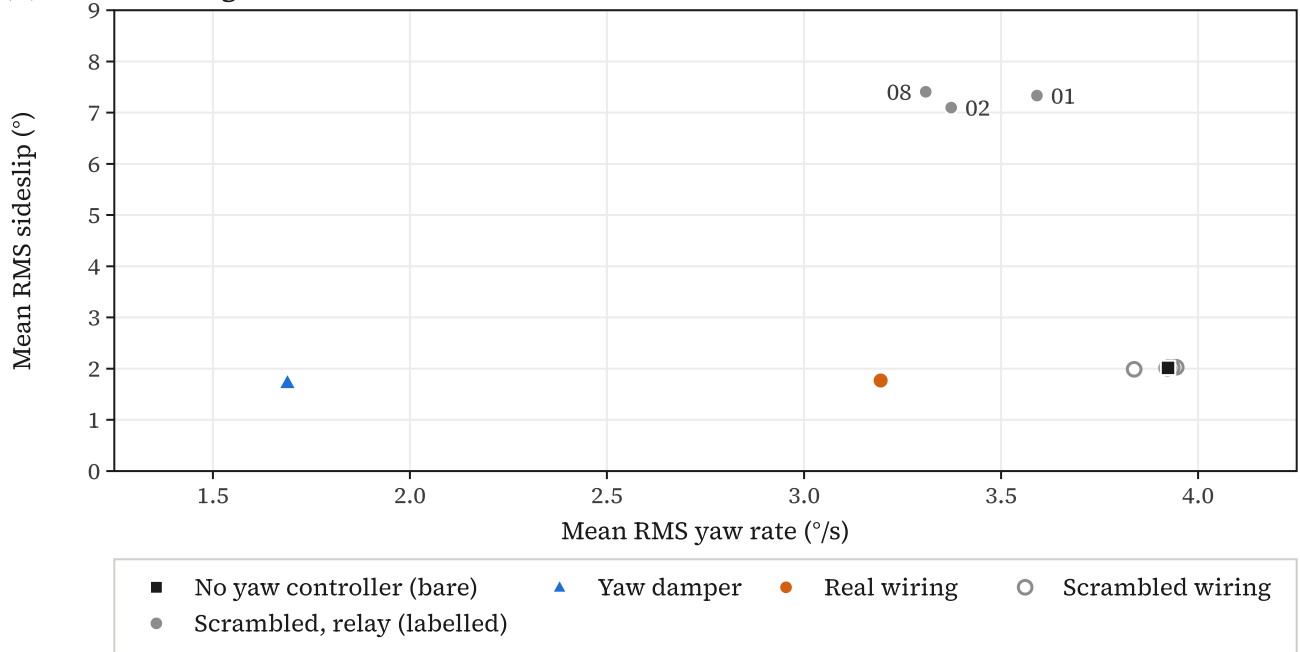
Figure 3. RMS sideslip against RMS yaw rate for every controller. Means over the 20 test seeds. A good yaw damper sits low on both axes. Filled grey points are scrambled wirings whose rudder was saturated in more than 90% of steps (relays); several scrambled wirings with K = 0 coincide with the bare airframe. Note the different sideslip scales: the axis in (a) is expanded, while (b) must also hold the relays. Bare: no yaw controller; on the six-degree-of-freedom model the wings-level roll hold common to every controller stays on.
