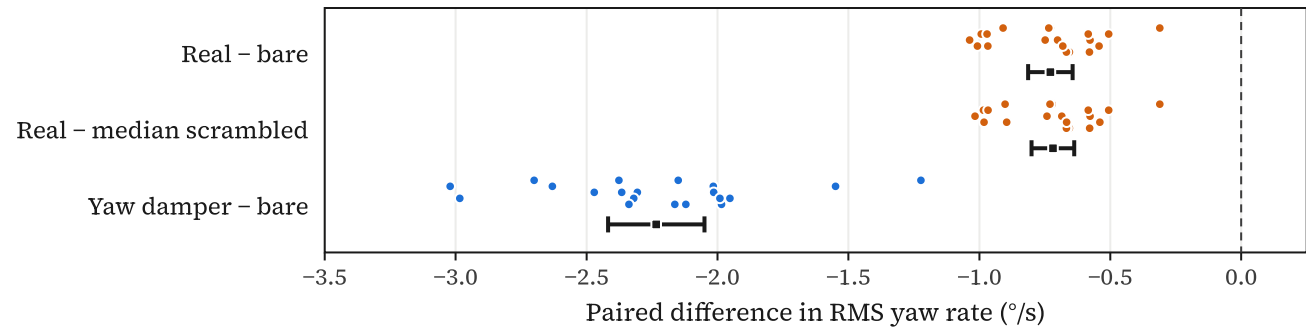
Figure 2. Paired differences in RMS yaw rate on the 20 held-out test seeds. Small dots: one per seed. Squares and bars: mean and 95% percentile bootstrap interval. Negative values favour the first-named controller. The real wiring helps on every seed; the yaw damper helps much more.
