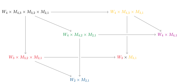
Figure 3: The punctured 3-cube diagram D_z associated with the object z = x_1 of degree 1, constructed from the right flow module W and the left flow module \mathcal{M}_{-,z} .
