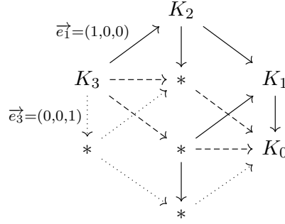
Figure 8: Composition of two n -chain maps f, g with n = 1 , in the special case where the source of f and the target of g are padded chains X_n, Y_0 . We embed f and g in [1]^2 \times [1]^n . The map f corresponds to the face x_3 = 0 , and g corresponds to x_1 = 1 . The dashed arrows represent the diagonal (the composition), and the dotted arrows represent the rest of the cube.
