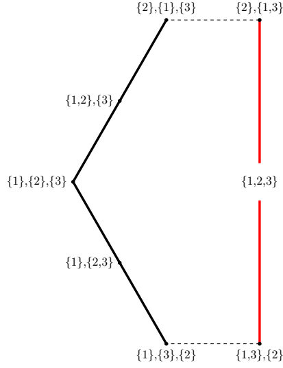
Figure 7: The half Permutohedron \frac{1}{2}P_3 . The vertices correspond to ordered partitions where 1 appears before or together with 3. The bold lines represent the corner. The diagonal \text{Diag}(P_3) is indicated in red. If we map from the category \frac{1}{2}[1]^3 to a category \mathcal{C} such that the map is zero outside the Spine, then the dotted lines correspond to the trivial part of the boundary \partial \frac{1}{2}P_3 .
