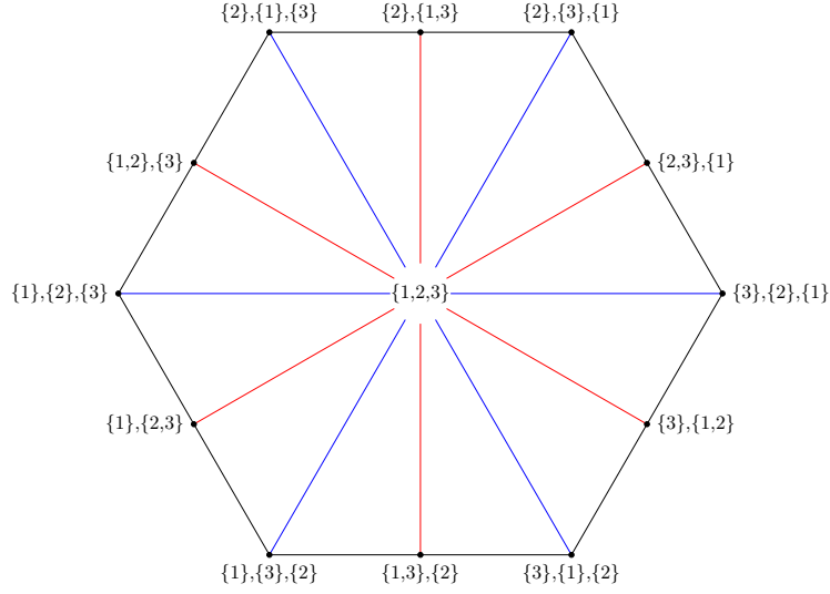
Figure 5: The mapping simplicial set \text{Hom}_{\text{Path } N[1]^3}(\emptyset, \{1, 2, 3\}) , which is the Permutohedron P_3 . The red lines divide the hexagon into six regions representing the maximal chains from \emptyset to \{1, 2, 3\} in [1]^3 . Each region has a kite shape, corresponding to the compositions of three morphisms. The blue lines subdivide the hexagon into a simplicial structure.
