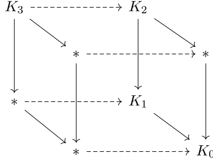
Figure 6: A spine 3-cube K , viewed as a morphism between spine 2-cubes. The dashed arrows represent morphisms between the faces (solid arrows), which are spine 2-cubes.
