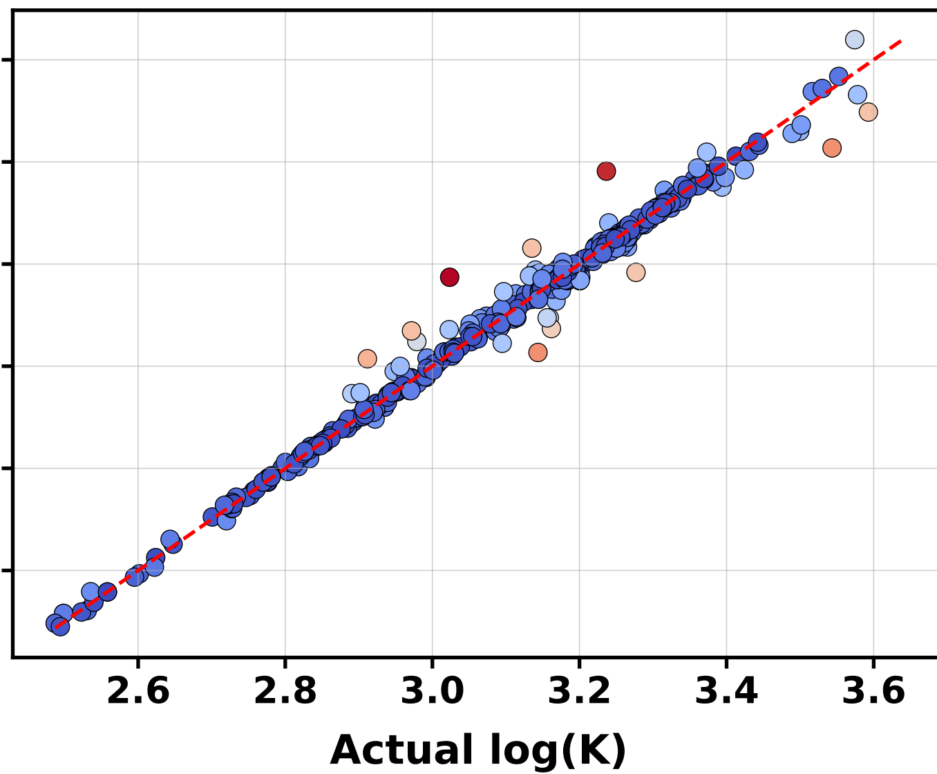
XGBoost
