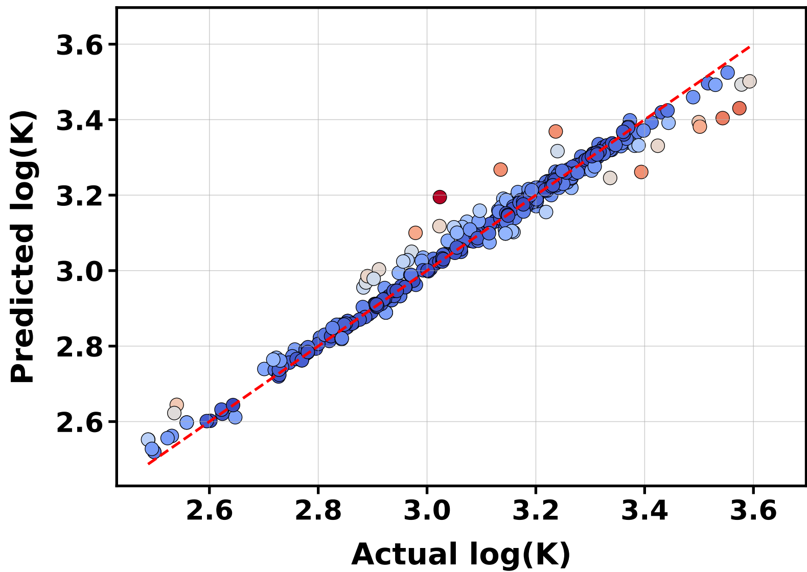
Random Forest
