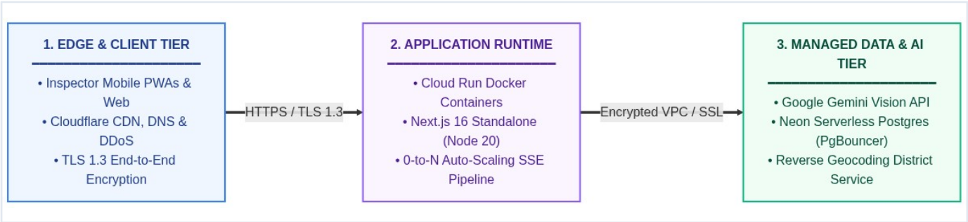
Figure 5: Multi-Cloud High-Availability Deployment Architecture
