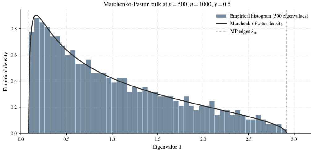
Figure 12: The ESD of \hat{\Sigma}_n = (1/n) \mathbf{X} \mathbf{X}^\top with iid Gaussian \mathbf{X} at p = 500 , n = 1000 (so y = 1/2 ). The histogram of all 500 eigenvalues from one realization closely matches the Marchenko-Pastur density (18) (solid curve). The dotted lines mark the support edges \lambda_{\pm} = (1 \pm \sqrt{y})^2 , with \lambda_- \approx 0.086 and \lambda_+ \approx 2.914 . Generated by notebooks/03_section3_demos.py .
