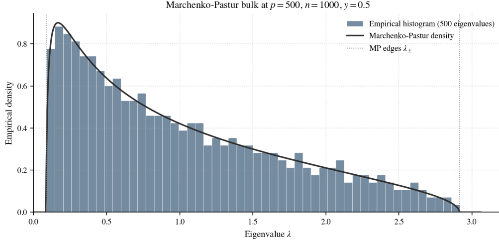
Figure 13: Single high-resolution realization at p = 500 , n = 1000 ( y = 1/2 ). The histogram of all 500 eigenvalues closely matches the Marchenko-Pastur density (20) (solid curve). The dotted lines mark the support edges \lambda_{\pm} = (1 \pm \sqrt{y})^2 \approx 0.086, 2.914 . Generated by notebooks/03_section3_demos.py .
