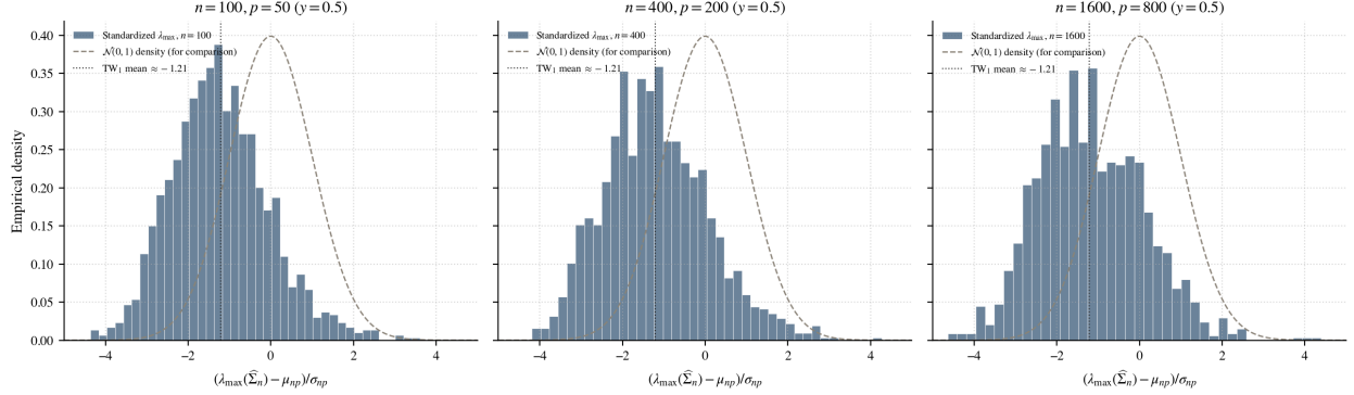
Figure 14: The Tracy-Widom edge in simulation. Each panel shows a histogram of the standardized top sample eigenvalue (\lambda_{\max}(\hat{\Sigma}_n) - \mu_{np})/\sigma_{np} over R = 1500 Monte Carlo trials, with p, n growing at fixed aspect ratio y = 1/2 . The histograms collapse to a common left-skewed shape that is not Gaussian (compare against the dashed \mathcal{N}(0, 1) density); the \text{TW}_1 mean \approx -1.21 is shown for reference. Generated by notebooks/03_section3_demos.py .
