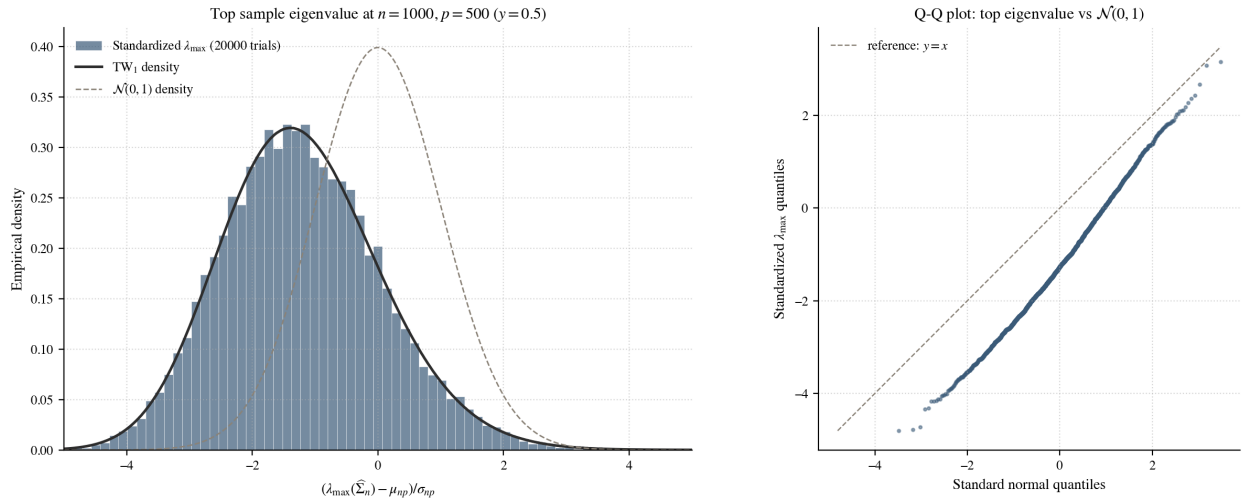
Figure 15: Direct comparison with the limiting Tracy-Widom density. Left: histogram of R = 20,000 standardized top sample eigenvalues at n = 1000, p = 500 ( y = 1/2 ), overlaid on the theoretical \text{TW}_1 density (solid sage curve) and the standard normal density (dashed) for contrast. The histogram tracks \text{TW}_1 closely and departs visibly from \mathcal{N}(0, 1) . Right: normal Q-Q plot of the same standardized samples against \mathcal{N}(0, 1) . The curvature, especially in the left tail where the \text{TW}_1 tail is heavier than Gaussian, confirms that the top-eigenvalue limit is not Gaussian. Generated by notebooks/03_section3_demos.py .
