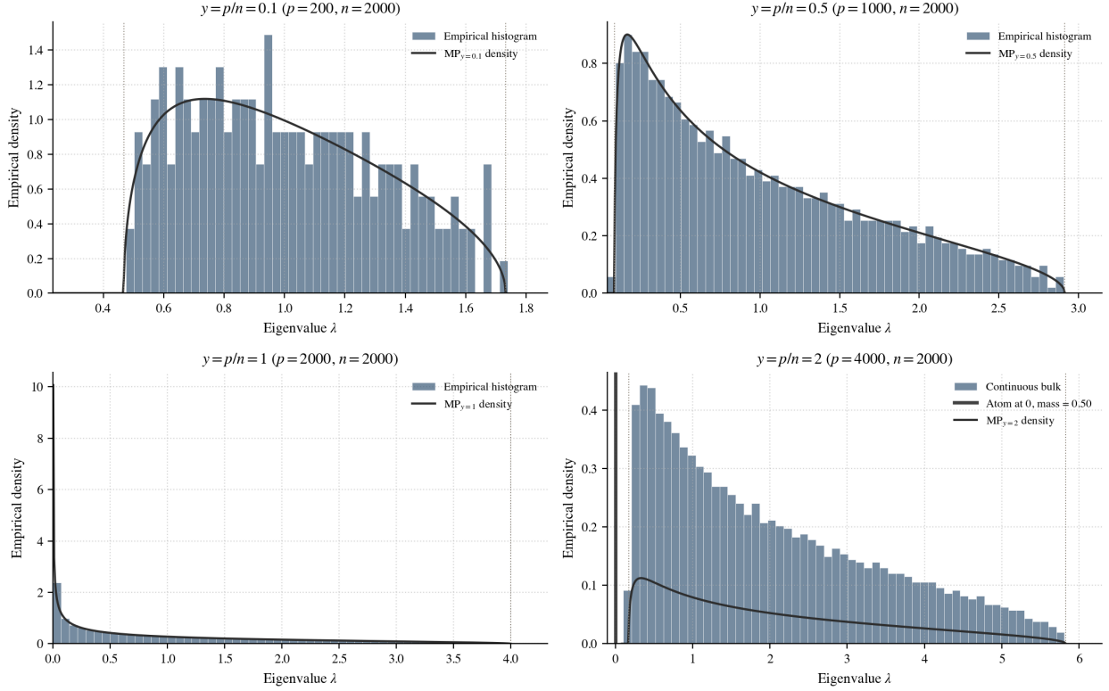
Figure 12: The Marchenko-Pastur law for four aspect ratios y \in \{0.1, 0.5, 1, 2\} . Each panel shows the histogram of p sample eigenvalues from a single realization of \hat{\Sigma}_n = (1/n) \mathbf{X} \mathbf{X}^\top with iid \mathcal{N}(0, 1) entries, overlaid on the theoretical MP_y density (20) (solid curve). For y > 1 (lower right) the law has an atom at zero of mass 1 - 1/y ; the histogram bar at \lambda = 0 reflects the p - n deterministic zero eigenvalues. Generated by notebooks/03_section3_demos.py .
