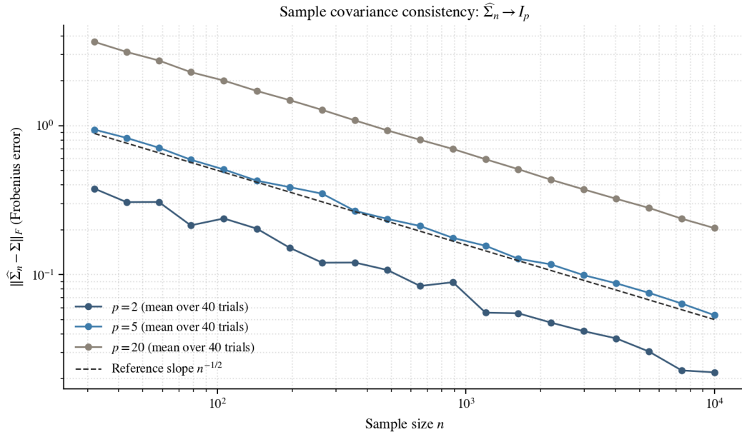
Figure 10: Sample covariance consistency in the low-dimensional regime. For \Sigma = I_p and iid Gaussian samples, the Frobenius error \|\widehat{\Sigma}_n - \Sigma\|_F averaged over 40 Monte Carlo trials is plotted against n (log-log axes) for three values of p . All three curves are parallel to the reference line of slope n^{-1/2} (dashed), confirming that the error vanishes at the expected rate. Theorem 3.2 below proves the entrywise version of this convergence.
