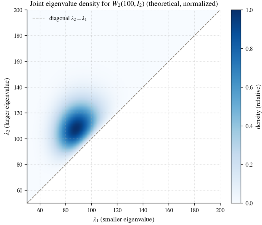
Figure 11: The theoretical joint eigenvalue density (15) of W_2(100, I_2) on the half-plane \lambda_1 \leq \lambda_2 . The density vanishes along the diagonal (dashed line) because of the (\lambda_2 - \lambda_1) factor; this dead zone is the analytic source of eigenvalue repulsion.
