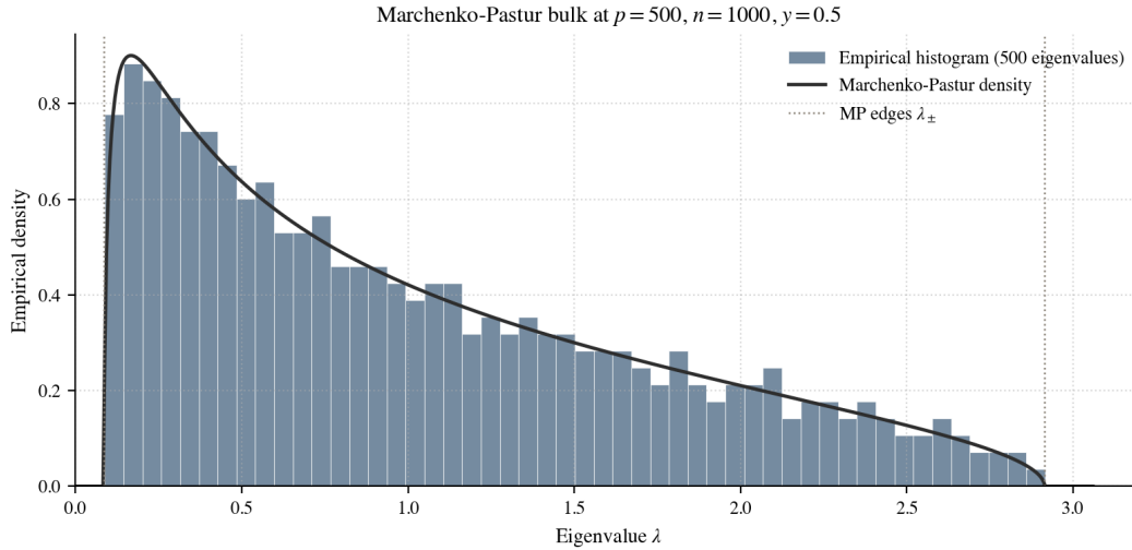
Figure 14: The ESD of \hat{\Sigma}_n = (1/n) \mathbf{X} \mathbf{X}^\top with iid Gaussian \mathbf{X} at p = 500 , n = 1000 (so y = 1/2 ). The histogram of all 500 eigenvalues from one realization closely matches the Marchenko-Pastur density (18) (solid curve). The dotted lines mark the support edges \lambda_{\pm} = (1 \pm \sqrt{y})^2 , with \lambda_- \approx 0.086 and \lambda_+ \approx 2.914 . Generated by notebooks/03_section3_demos.py .
