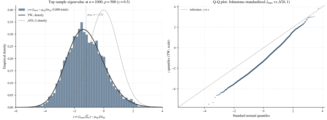
Figure 14: Direct comparison with the limiting Tracy-Widom distribution. For each of R = 5000 trials we compute \lambda_{\max}((1/n) \mathbf{X} \mathbf{X}^\top) with iid \mathcal{N}(0, 1) entries at n = 1000 , p = 500 ( y = 1/2 ), and form the Johnstone-standardized statistic z = (\lambda_{\max} - \mu_{np}) / \sigma_{np} . The two panels show the raw z -values without any further normalization, so the empirical objects retain the \text{TW}_1 location and scale. Left: histogram of z overlaid on the theoretical \text{TW}_1 density (solid sage curve) and the standard normal density (dashed) for contrast. The \text{TW}_1 bulk is shifted to the left of the Gaussian; its mean (vertical dotted marker at -1.21 ) sits well below 0, and its mode at \approx -1.77 is even further left. The histogram tracks \text{TW}_1 closely. Right: Q-Q plot of every z sample against \mathcal{N}(0, 1) quantiles, with the y = x reference drawn for context. Because \text{TW}_1 has different mean, scale, and shape than \mathcal{N}(0, 1) , the points are not expected to lie on y = x ; they sit below it at the bulk (consequence of \text{TW}_1 's negative mean) and cross above it at the upper extreme (consequence of \text{TW}_1 's heavier right tail). Generated by notebooks/03_section3_demos.py .
