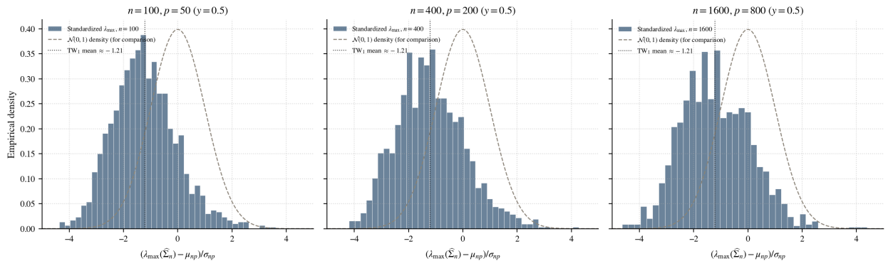
Figure 13: The Tracy-Widom edge in simulation. Each panel shows a histogram of the standardized top sample eigenvalue (\lambda_{\max}(\hat{\Sigma}_n) - \mu_{np}) / \sigma_{np} over R = 1500 Monte Carlo trials, with p, n growing at fixed aspect ratio y = 1/2 . The histograms collapse to a common left-skewed shape that is not Gaussian (compare against the dashed \mathcal{N}(0, 1) density); the \text{TW}_1 mean \approx -1.21 is shown for reference. Generated by notebooks/03_section3_demos.py .
