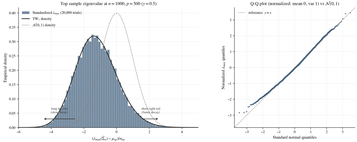
Figure 14: Direct comparison with the limiting Tracy-Widom density. Left: histogram of R = 20,000 standardized top sample eigenvalues at n = 1000, p = 500 ( y = 1/2 ), overlaid on the theoretical TW_1 density (solid sage curve) and the standard normal density (dashed) for contrast. The TW_1 shape is clearly asymmetric: a long left tail extending below the mode at \approx -1.6 (reflecting many “pushed-back” configurations of \lambda_{\max} into the bulk) versus a shorter right tail (reflecting the rarer excursions above the typical edge). The Gaussian density is symmetric and centered at zero with smaller spread, and the histogram tracks TW_1 rather than \mathcal{N}(0, 1) . Right: Q-Q plot of the same standardized samples, after a further centering and scaling to mean 0 and variance 1 so that the comparison isolates shape from location (this is the convention used in Genzer (2025, Fig. 7)). The marked curvature, especially in the left tail where TW_1 extends well below the Gaussian quantile and in the right tail where it falls short, certifies that the top-eigenvalue limit is not Gaussian. Generated by notebooks/03_section3_demos.py .
