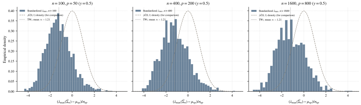
Figure 12: The Tracy-Widom edge in simulation. Each panel shows a histogram of the standardized top sample eigenvalue (\lambda_{\max}(\hat{\Sigma}_n) - \mu_{np})/\sigma_{np} over R = 1500 Monte Carlo trials, with p, n growing while y = p/n = 1/2 is held fixed. The histograms are unambiguously non-Gaussian and become more sharply defined as n grows, converging to the Tracy-Widom \text{TW}_1 shape predicted by Theorem 3.7. The asymmetry (heavier left tail, lighter right) is the visible signature of \text{TW}_1 . Generated by notebooks/03.section3.demos.py .
