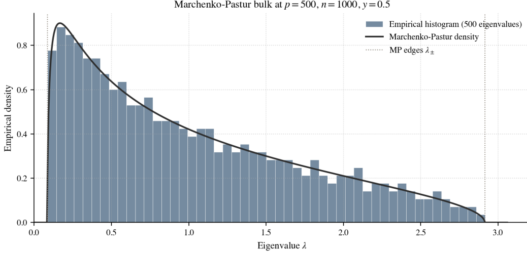
Figure 11: Empirical eigenvalue distribution of the null sample covariance matrix \hat{\Sigma}_n = (1/n) \mathbf{X} \mathbf{X}^\top with iid Gaussian \mathbf{X} , at p = 500 , n = 1000 (so y = 1/2 ). The histogram of all 500 eigenvalues from one realization matches the Marchenko-Pastur density (12) closely; the dotted lines mark the support edges \lambda_{\pm} = (1 \pm \sqrt{y})^2 , with \lambda_- \approx 0.086 and \lambda_+ \approx 2.914 . Generated by notebooks/03_section3_demos.py .
