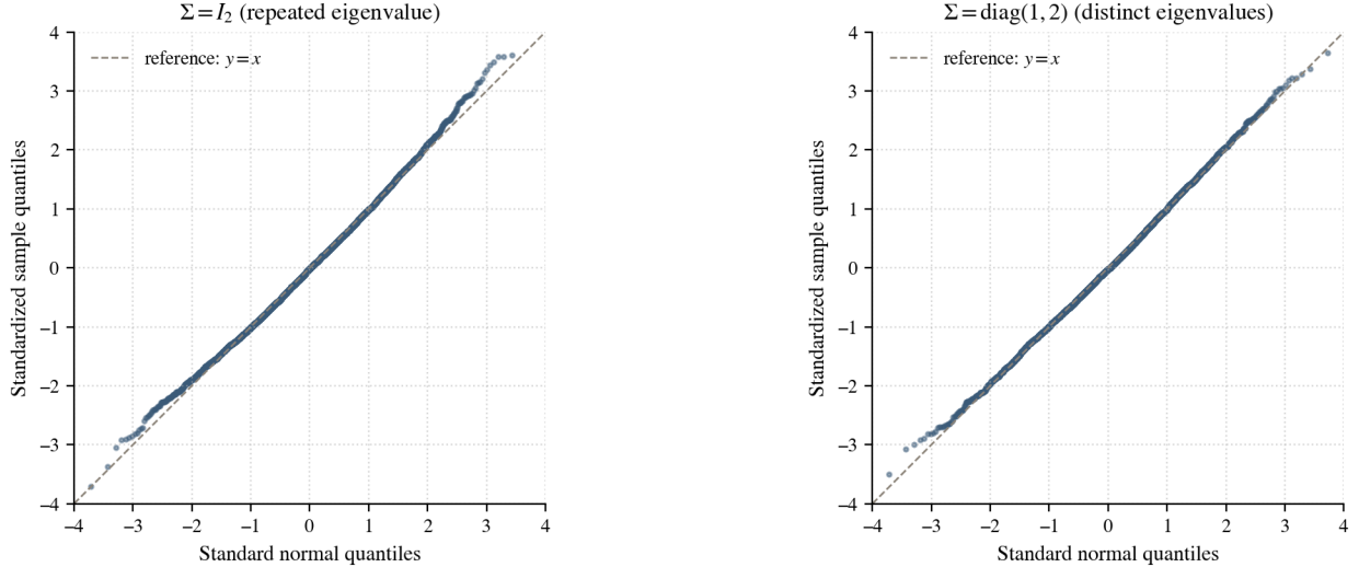
Figure 10: Normal Q-Q plots for the standardized top sample eigenvalue \sqrt{n}(\lambda_{\max}(\hat{\Sigma}_n) - \lambda_{\max}(\Sigma)) , 5000 Monte Carlo trials with n = 500 . Left: \Sigma = I_2 (repeated population eigenvalues). The systematic departure from the dashed reference line, especially the heavier right tail and the curve at the left, reflects the non-Gaussian GOE limit. Right: \Sigma = \text{diag}(1, 2) (distinct population eigenvalues). The points lie close to the reference line, confirming the Gaussian limit in equation (11). Generated by notebooks/03_section3_demos.py .
