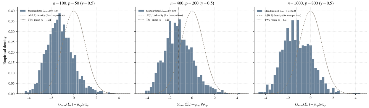
Figure 13: The Tracy-Widom edge in simulation. Each panel shows a histogram of the standardized top sample eigenvalue (\lambda_{\max}(\hat{\Sigma}_n) - \mu_{np})/\sigma_{np} over R = 1500 Monte Carlo trials, with p, n growing at fixed aspect ratio y = 1/2 . The histograms collapse to a common left-skewed shape that is not Gaussian (compare against the dashed \mathcal{N}(0, 1) density); the \text{TW}_1 mean \approx -1.21 is shown for reference. Generated by notebooks/03_section3_demos.py .
