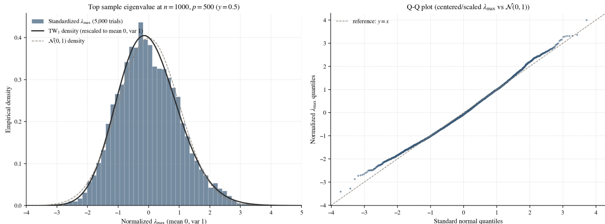
Figure 14: Direct comparison with the limiting Tracy-Widom density, following the procedure of Genzer (2025, Fig. 7 and Listing 7) . For each of R = 5000 trials we compute \lambda_{\max}((1/n) \mathbf{X} \mathbf{X}^\top) with iid \mathcal{N}(0, 1) entries at n = 1000 , p = 500 ( y = 1/2 ), then standardize by the sample mean and sample standard deviation. Left: histogram of the standardized values, overlaid on the theoretical \text{TW}_1 density rescaled to mean 0 and variance 1 (solid sage curve) and the standard normal density (dashed). The empirical histogram tracks the rescaled \text{TW}_1 closely; its mode sits at \approx -0.4 (the mode of \text{TW}_1 after the same rescaling), well to the left of the Gaussian mode at 0. Right: Q-Q plot of every standardized sample against \mathcal{N}(0, 1) quantiles. The right tail visibly rises above the y = x reference, with the most extreme \lambda_{\max} samples reaching z \approx 4 while the matching Gaussian quantiles are only \approx 3 ; the left tail bends in the opposite sense. Both panels confirm that the top-eigenvalue limit is non-Gaussian, with a heavier right tail than \mathcal{N}(0, 1) . Generated by notebooks/03_section3_demos.py .
