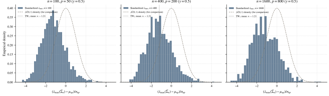
Figure 14: Histogram of z = (\lambda_{\max}(\widehat{\Sigma}_n) - \mu_{np})/\sigma_{np} at three growing (n, p) pairs with fixed aspect ratio y = 1/2 ; R = 1500 Monte Carlo trials per panel. The standard normal density (dashed) and the \text{TW}_1 mean ( \approx -1.21 , dotted) are shown for reference. Generated by notebooks/03_section3_demos.py .
