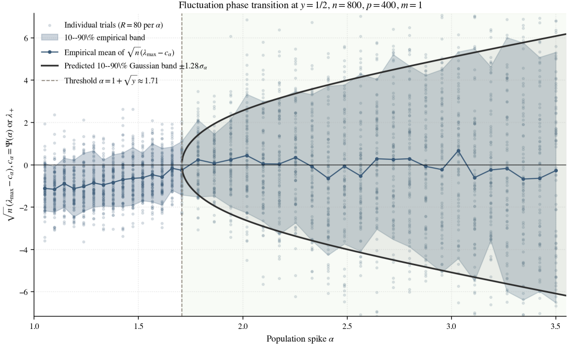
Figure 20: Fluctuation phase transition swept across the spike strength at y = 1/2 , n = 800 , p = 400 , m = 1 . For each \alpha in a grid covering both sides of the threshold 1 + \sqrt{y} , we run R = 80 replications and record \sqrt{n}(\lambda_{\max}(\hat{\Sigma}_n) - c_\alpha) , where c_\alpha = \Psi(\alpha) above the threshold and c_\alpha = \lambda_+ below it. The translucent dots are individual trials, the green curve is the empirical mean, and the shaded green band is the 10–90% empirical envelope. The black band is the Theorem 4.3 prediction \pm 1.28\sigma_\alpha on the fundamental segment (shaded), which collapses to zero at the threshold. Below the threshold the empirical spread is tight near zero because the genuine edge fluctuations live on the smaller p^{-2/3} scale of Theorem 4.4, invisible at the \sqrt{n} resolution of this plot. Generated by notebooks/04_section4_demos.py .
