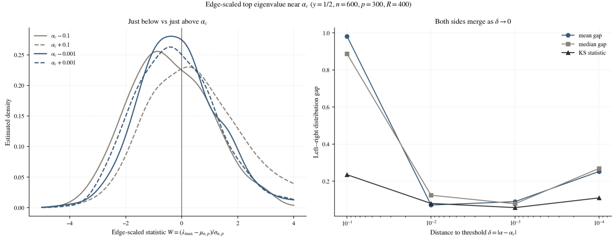
Figure 22: Edge-scaled top eigenvalue W = (\lambda_{\max} - \mu_{n,p}) / \sigma_{n,p} near the threshold, at y = 1/2 , n = 600 , p = 300 , R = 400 . Left: kernel-density estimates just below ( \alpha_c - \delta , solid) and just above ( \alpha_c + \delta , dashed) the threshold; at \delta = 10^{-1} the two sides are clearly distinct, while at \delta = 10^{-3} they coincide. Right: the left-right gap in mean, median, and Kolmogorov-Smirnov distance collapses as \delta \rightarrow 0 ; the small residual at \delta = 10^{-4} , where the two distributions are effectively identical, is sampling noise. Generated by notebooks/04_section4_demos.py .
