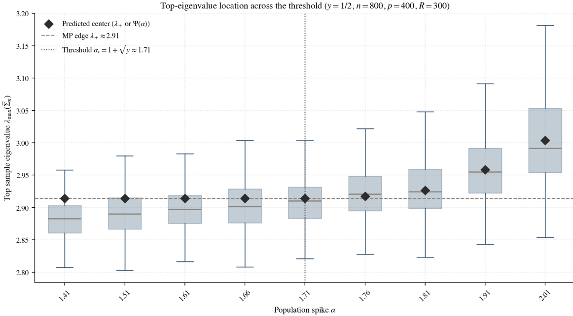
Figure 21: Top sample eigenvalue \lambda_{\max}(\hat{\Sigma}_n) as the spike crosses the threshold, at y = 1/2 , n = 800 , p = 400 , with R = 300 replications per spike (whiskers shown, outliers suppressed). Diamonds mark the predicted location of Theorem 4.2: the Marchenko-Pastur edge \lambda_+ for \alpha \leq \alpha_c and \Psi(\alpha) for \alpha > \alpha_c . Because \Psi'(\alpha_c) = 0 , the prediction leaves the edge tangentially, and the boxes cross \alpha_c \approx 1.71 without a visible jump. Generated by notebooks/04_section4_demos.py .
