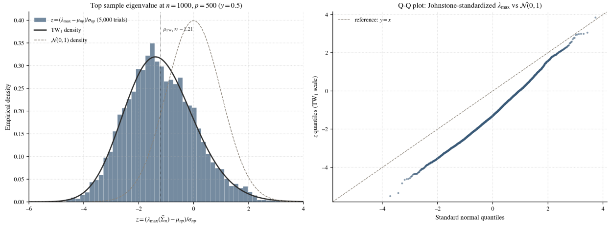
Figure 14: Direct comparison of the empirical z = (\lambda_{\max} - \mu_{np})/\sigma_{np} at n = 1000, p = 500 ( y = 1/2 , R = 5000 trials) with the limiting Tracy-Widom distribution. Left: histogram of z against the theoretical \text{TW}_1 density (solid) and the standard normal density (dashed); the \text{TW}_1 bulk is centred on its mean \approx -1.21 , well to the left of the Gaussian. Right: Q-Q plot of z against \mathcal{N}(0, 1) quantiles. The curve sits below the y = x reference at the bulk ( \text{TW}_1 's negative mean) and crosses above it at the upper extreme ( \text{TW}_1 's heavier right tail). Generated by notebooks/03_section3_demos.py .
