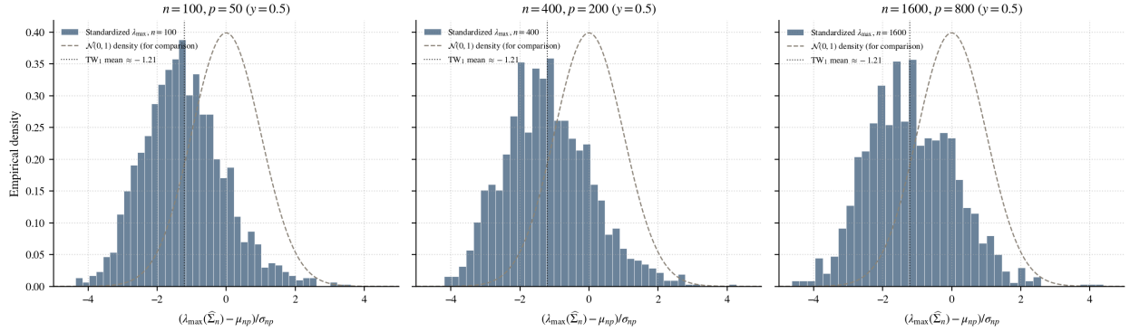
Figure 13: Histogram of z = (\lambda_{\max}(\hat{\Sigma}_n) - \mu_{np})/\sigma_{np} at three growing (n, p) pairs with fixed aspect ratio y = 1/2 ; R = 1500 Monte Carlo trials per panel. The standard normal density (dashed) and the \text{TW}_1 mean ( \approx -1.21 , dotted) are shown for reference. Generated by notebooks/03_section3_demos.py .
