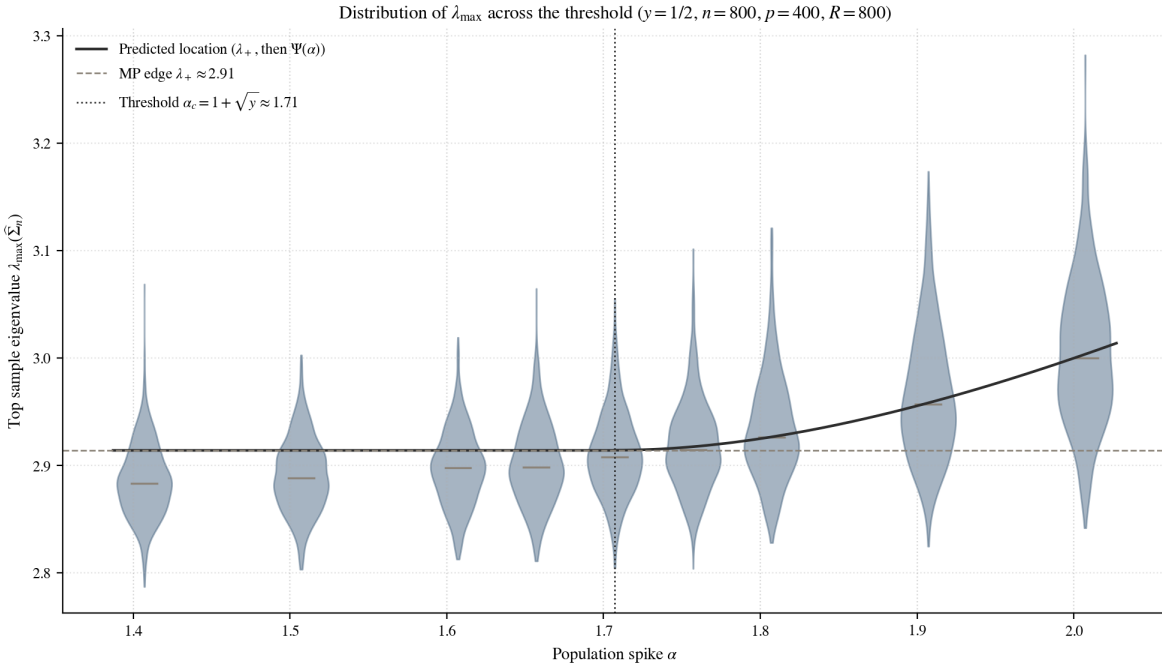
Figure 21: Distribution of the top sample eigenvalue \lambda_{\max}(\hat{\Sigma}_n) as the spike crosses the threshold, at y = 1/2 , n = 800 , p = 400 , with R = 800 replications per spike (each violin is a kernel-density estimate; the bar marks the median). The solid curve is the predicted location of Theorem 4.2: the Marchenko-Pastur edge \lambda_+ for \alpha \leq \alpha_c and \Psi(\alpha) for \alpha > \alpha_c . Below \alpha_c the distribution is tight and pinned at the edge; above it the distribution lifts along \Psi(\alpha) , broadens, and becomes symmetric. Generated by notebooks/04_section4_demos.py .
