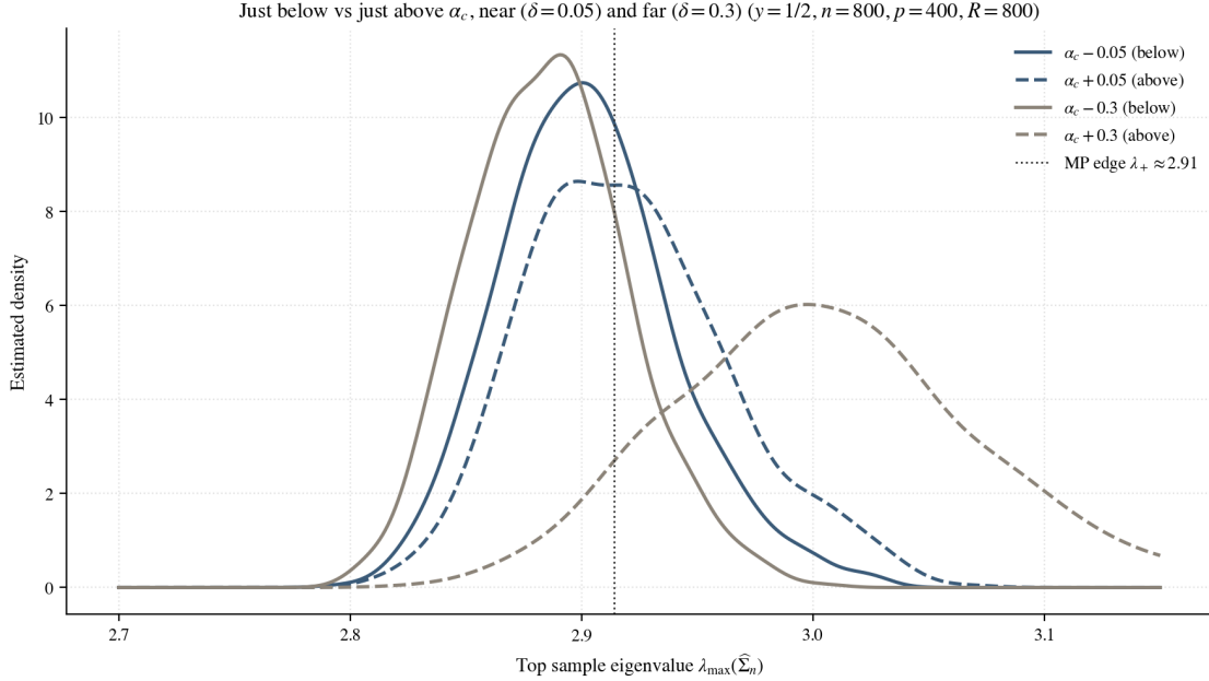
Figure 22: Raw distributions of \lambda_{\max}(\hat{\Sigma}_n) just below ( \alpha_c - \delta , solid) and just above ( \alpha_c + \delta , dashed) the threshold, at y = 1/2 , n = 800 , p = 400 , R = 800 . At the small distance \delta = 0.05 (dark) the two sides coincide; at the large distance \delta = 0.30 (grey) the supercritical side has lifted away from the edge while the subcritical side stays pinned at \lambda_+ . No rescaling is applied: the horizontal axis is the eigenvalue itself. Generated by notebooks/04_section4_demos.py .
