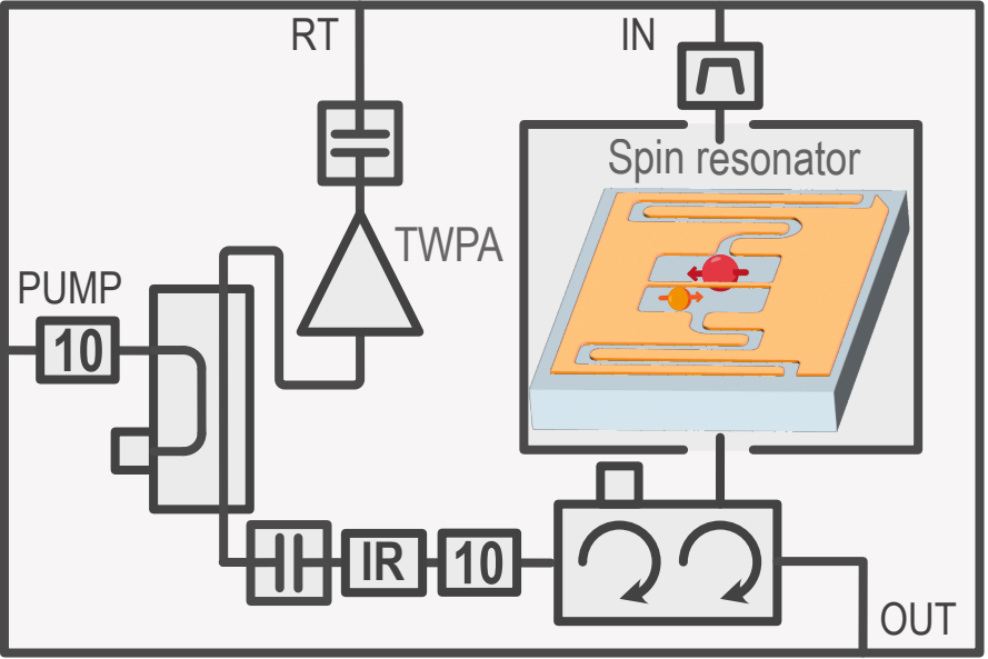
Setup 2: Transmission
