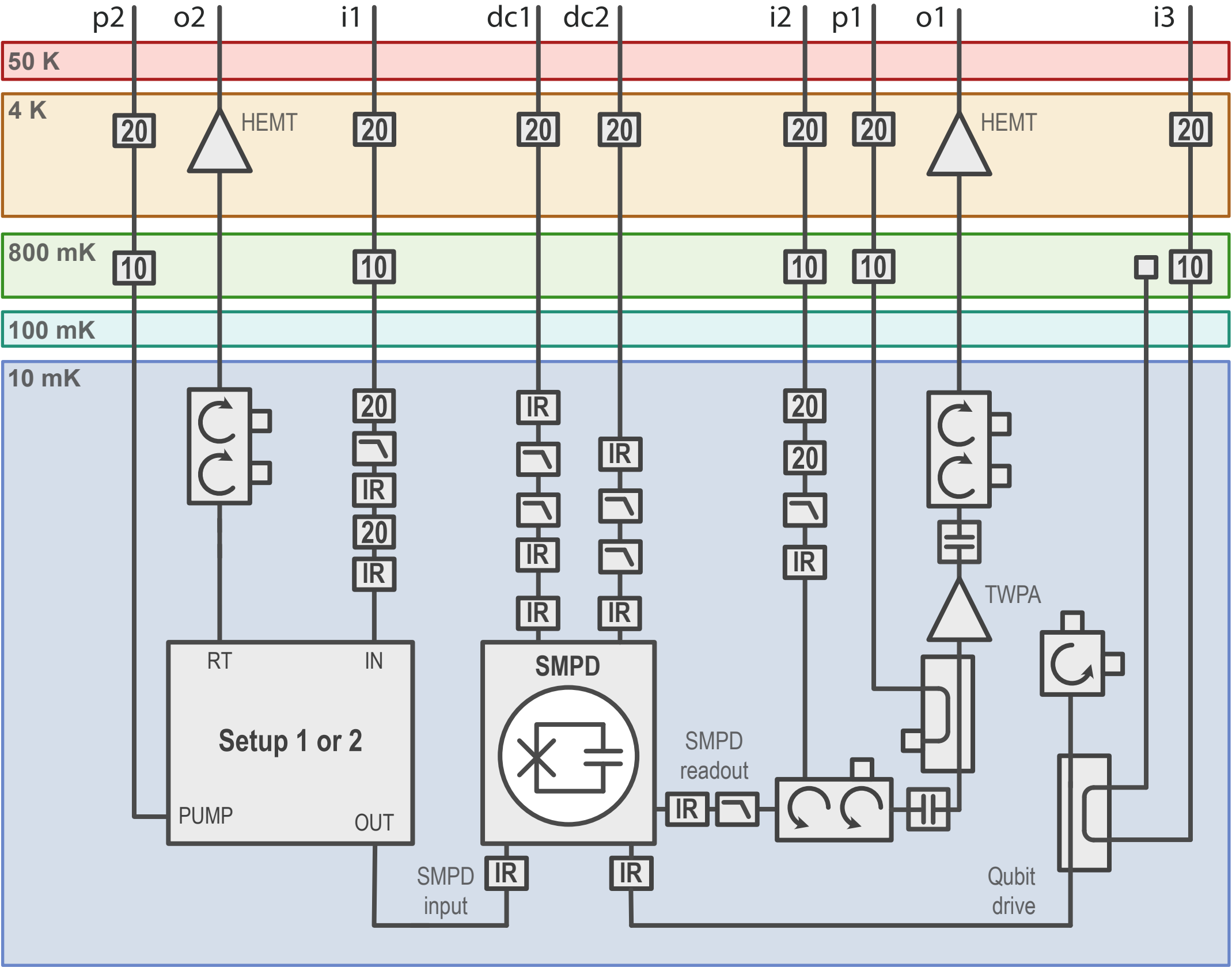
Setup 2: Transmission
