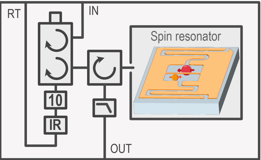
Setup 1: Reflection
