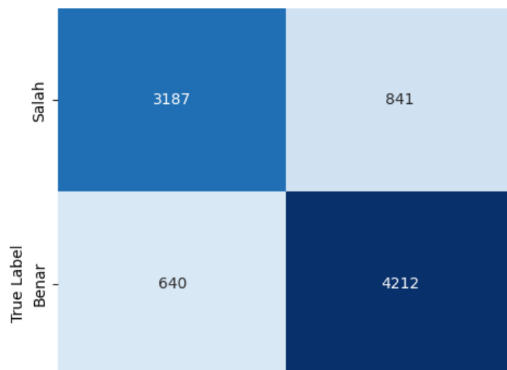
Gambar 4.6 Confusion Matrix Model Random Forest
