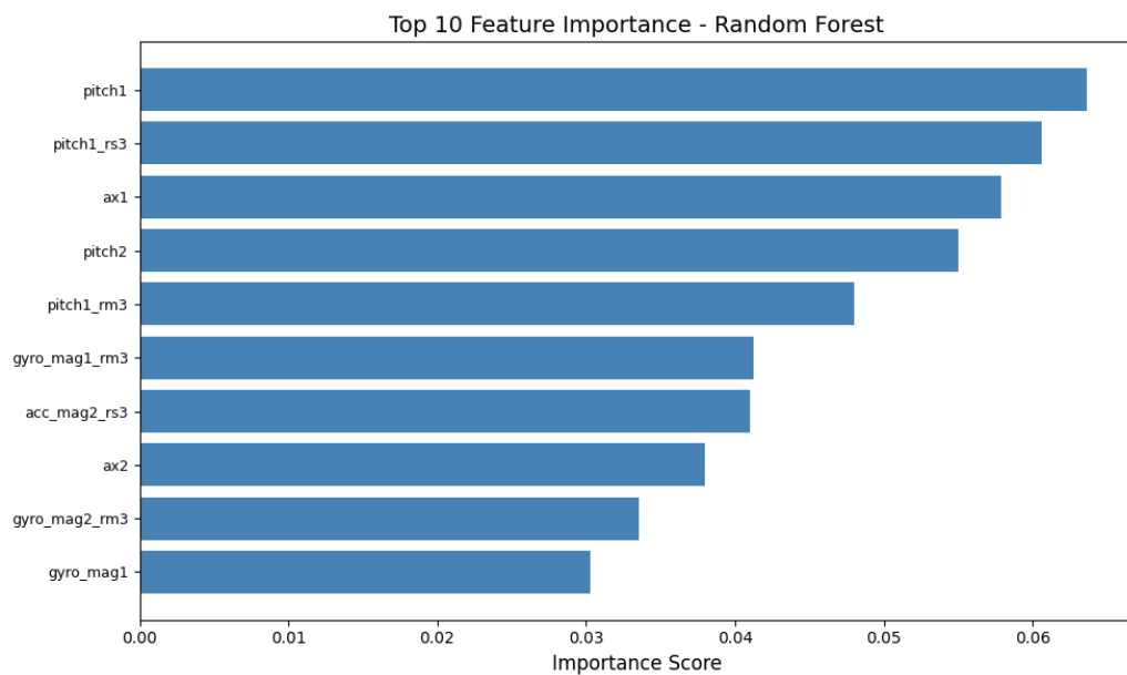
Gambar 4.7 Feature Importance Model Random Forest
