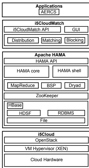
Figure 0.1: Framework Architecture
