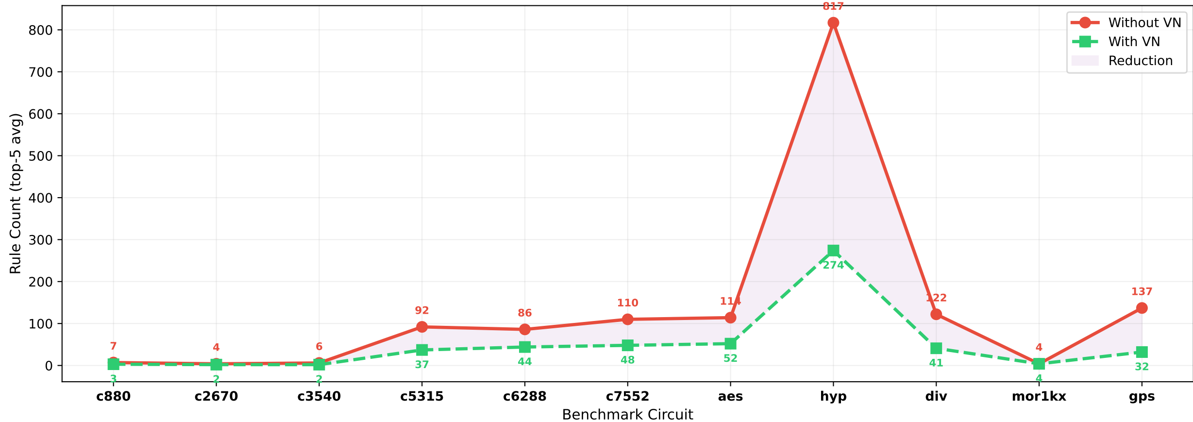
Decision Tree Rule Count: Before vs After Virtual Node
