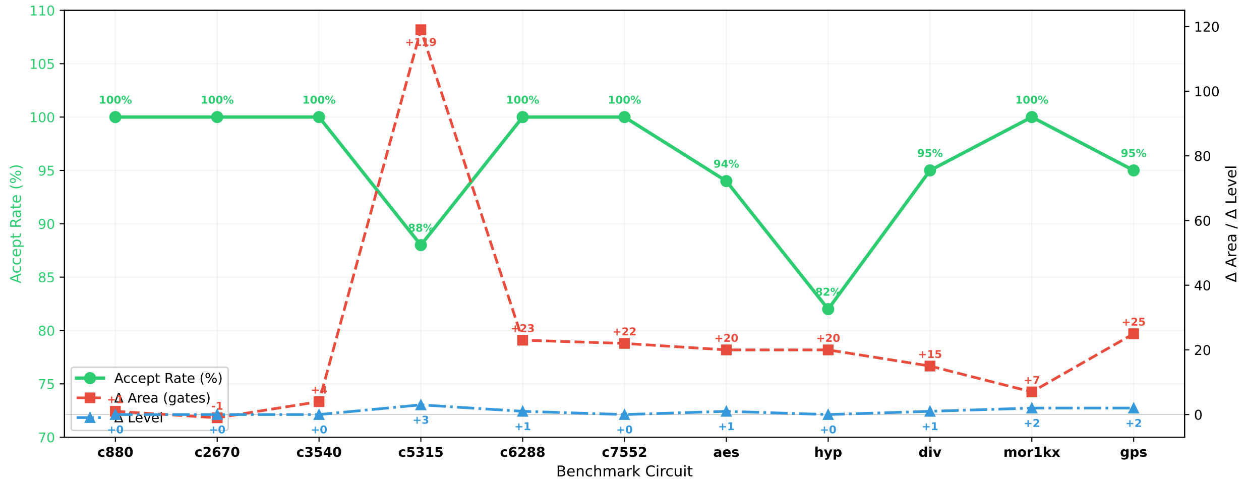
Hardware Trojan Patching: Accept Rate, Area Overhead, and Level Overhead
