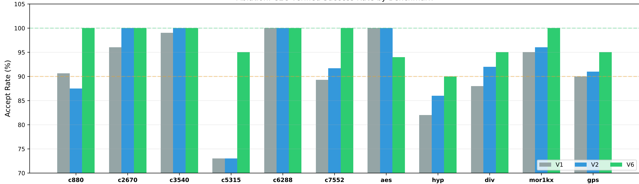
Ablation: CEC-Verified Success Rate by Benchmark
