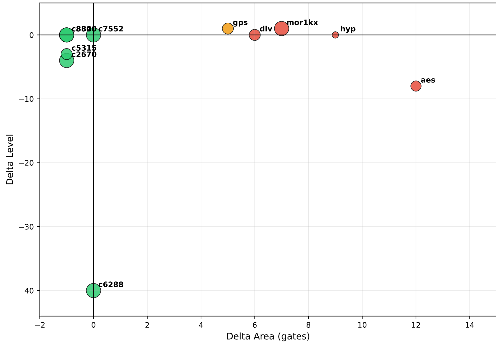
v6 Area / Level Trade-off by Benchmark
