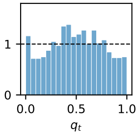
VUAG.L GARCH(1,1)
