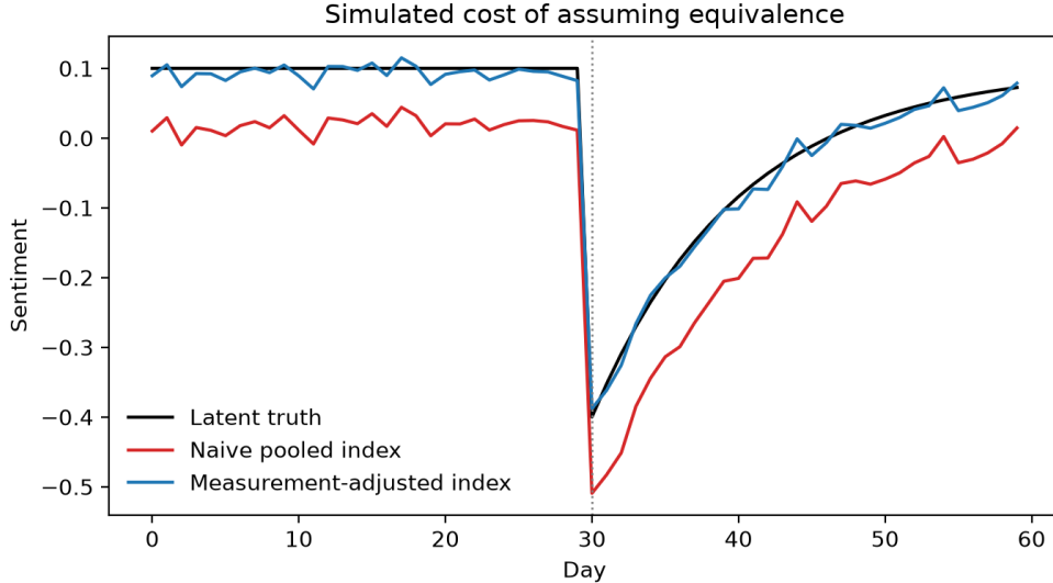
Figure 6: One simulation run (seed 20261201; parameters fixed ex ante, shipped with the code). The naive pooled index distorts the event shift and reports the wrong sign of aggregate sentiment on 13 of 60 days in this run; the measurement-adjusted index recovers the latent truth with no wrong sign day in this run. Here the true event shift is -0.332 ; the naive index estimates -0.369 and the adjusted index -0.326 .
