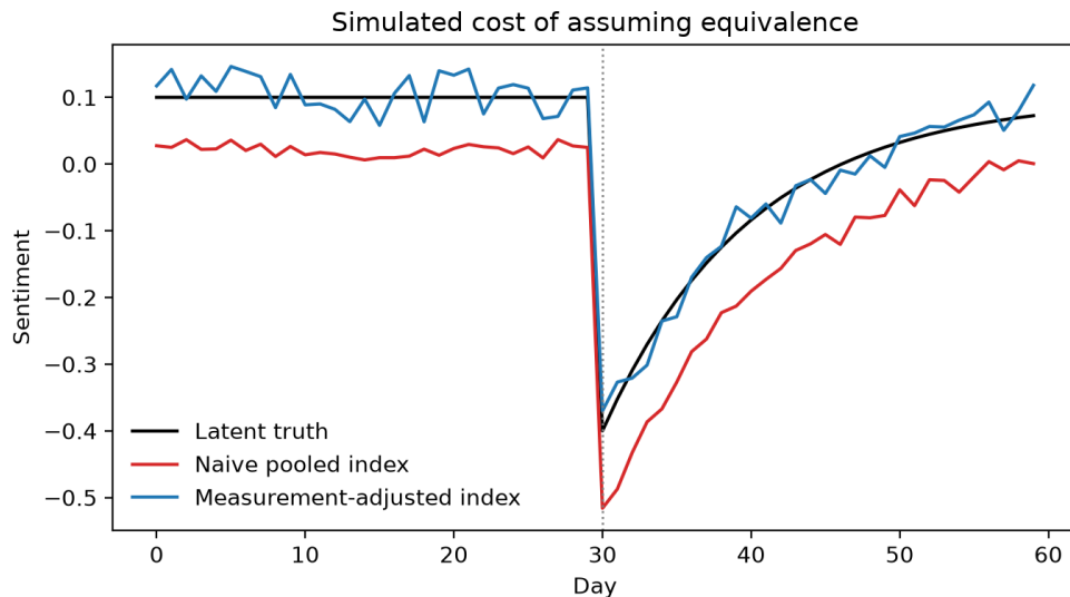
Figure 6: Prototype simulation run with illustrative parameters (seed 20261201; final parameters to be pre-registered). The naive pooled index distorts the event shift and reports the wrong sign of aggregate sentiment on 10 of 60 simulated days; the measurement-adjusted index recovers the latent truth. In this run the true event shift is -0.332 ; the naive index estimates -0.374 and the adjusted index -0.334 .
