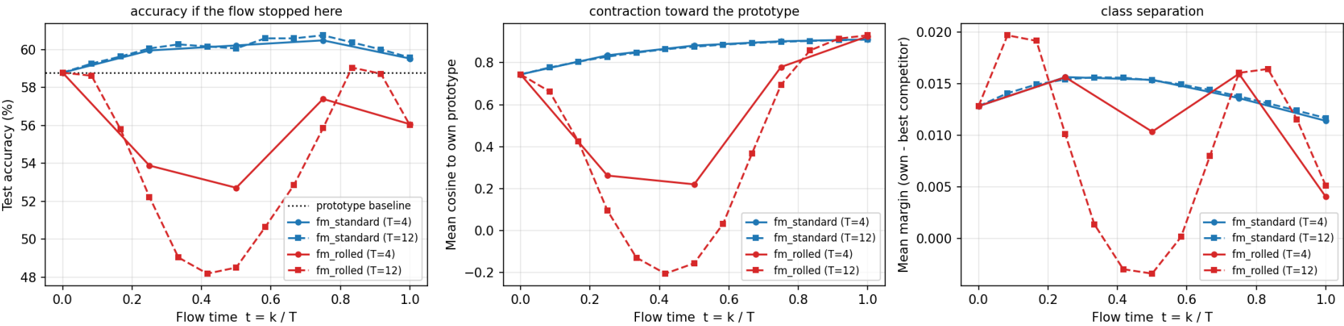
dtd / resnet18: metrics along the flow (K=full)
