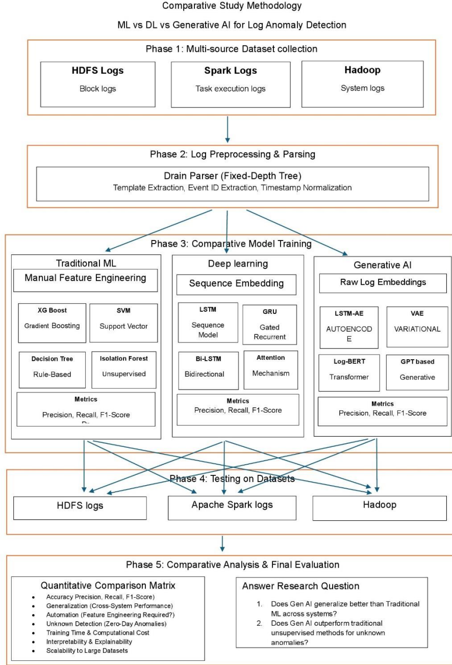
Figure 1 Methodology
